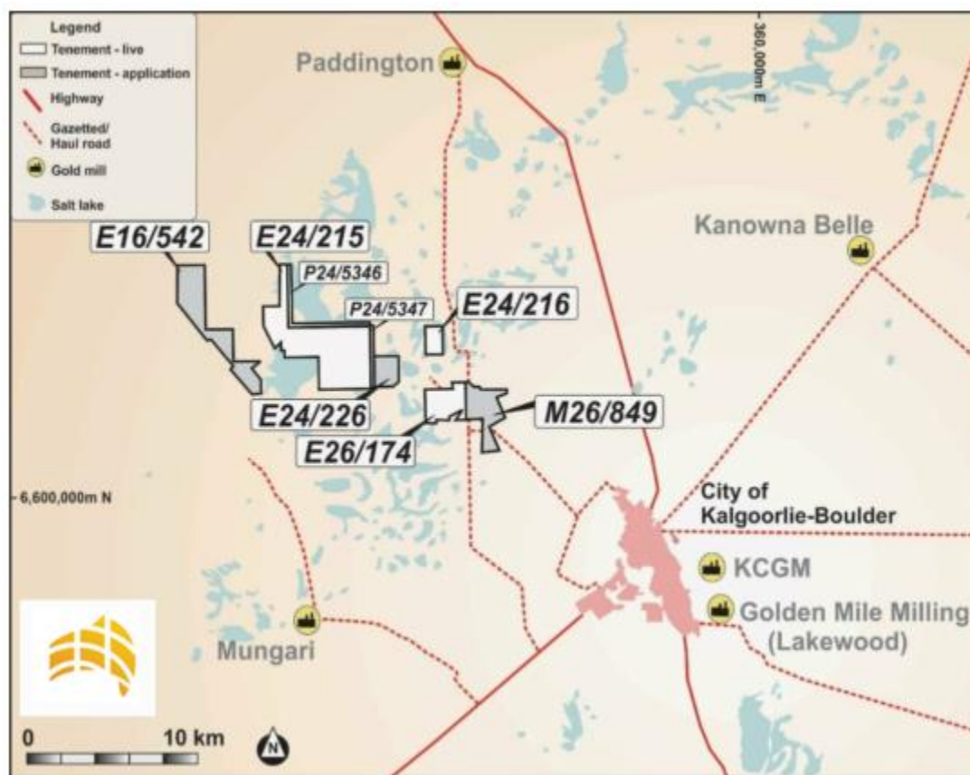
Figure 10. FAU tenure around the Kalgoorlie Region, including Gimlet
