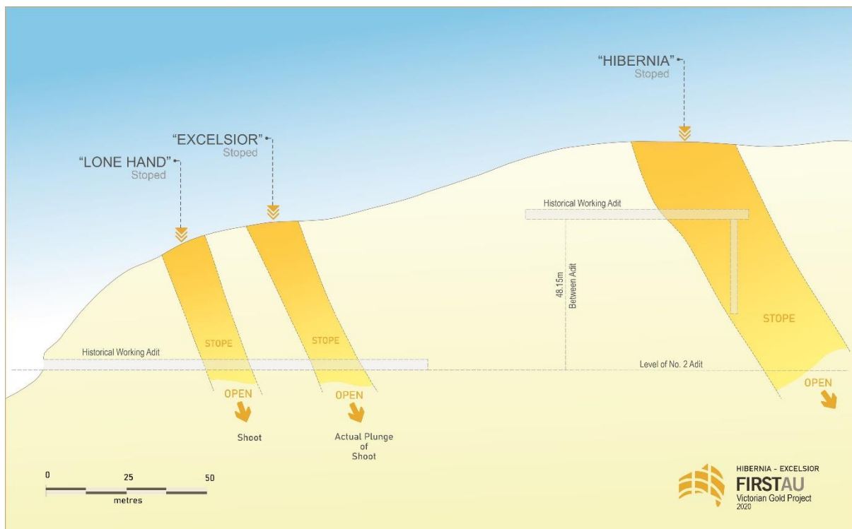
Figure 6: Long section of historical workings across the Hibernia mine corridor - View West
