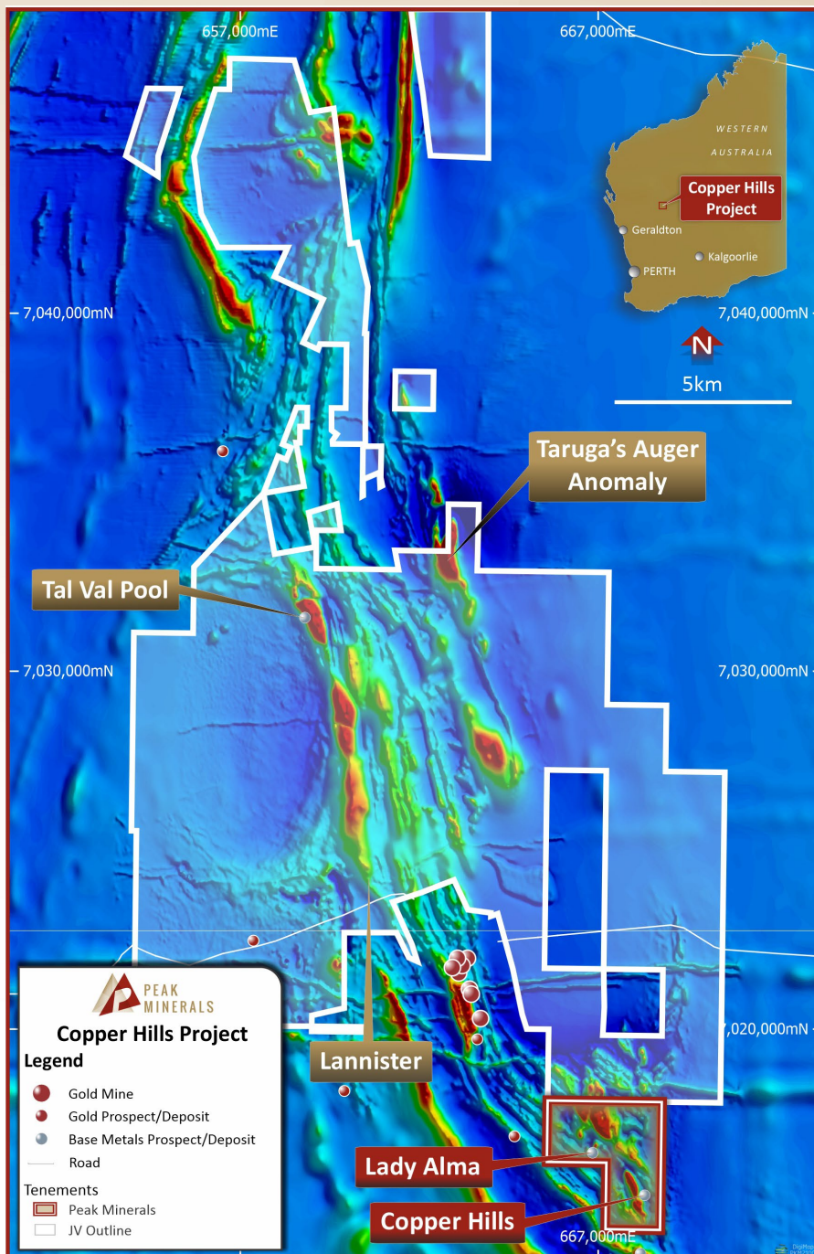
Figure 1: Magnetic TMI image with outline of JV. Note the red zones represent high magnetism and at Lady Alma and Copper Hills this maps out the intrusive units.
