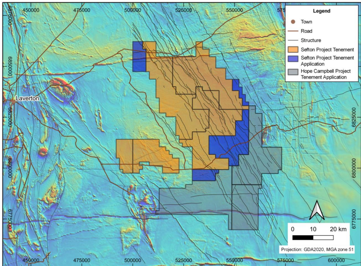
Figure 1. Sefton Project tenements and the newly applied for Hope Campbell tenements. Background image is a regional magnetic image and major structures.
