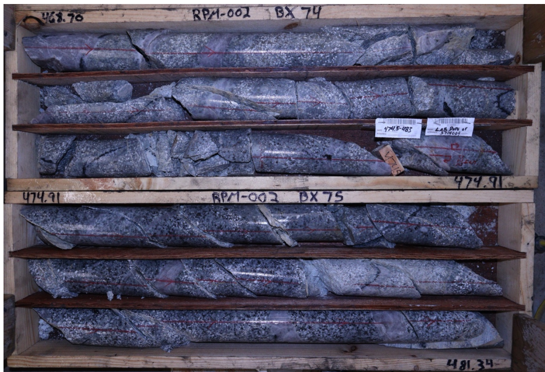
Figure 3: RPM-002 - Typical low sulfide quartz-tourmaline-sulfide veining in phyllic altered granitic intrusive
