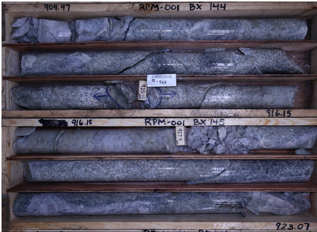
Figure 4: RPM-001 - Quartz veining with minor sulfide in phyllic altered granitic intrusive
