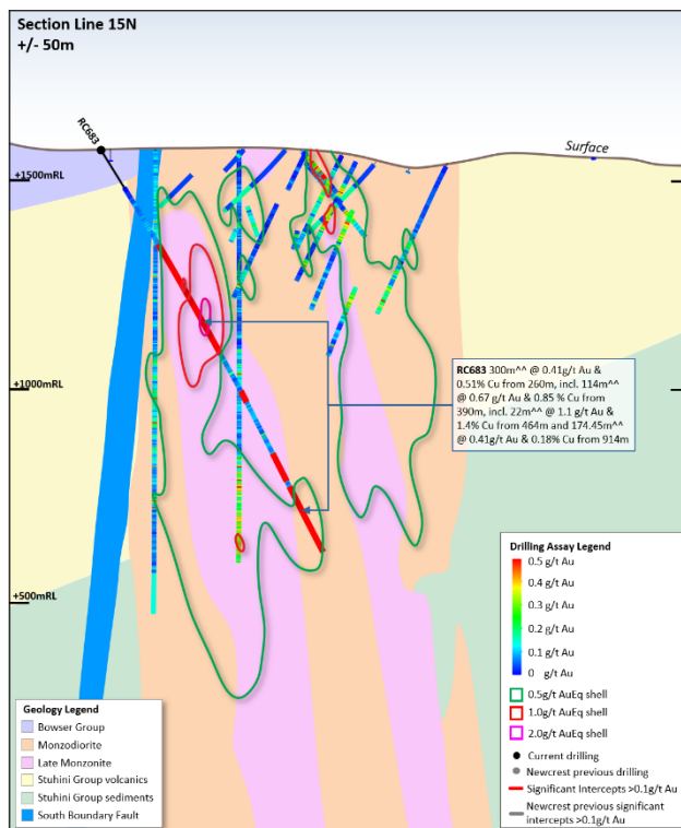
Figure 12. Schematic cross section of RC683 ( Section Line 15N ) showing Newcrest and Imperial drill holes and Newcrest intercepts (drill intercepts have been reported in Appendix 1 of this report, and in prior Newcrest exploration releases) 0.5 g/t AuEq, 1 g/t AuEq and 2 g/t AuEq shell projections generated from Leapfrog model. Due to window size (+/- 50m) and section orientation (150°) hole may appear on multiple sections.
