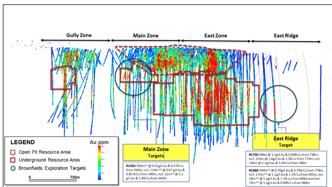
Figure 2. Long section view of the Red Chris porphyry corridor showing drill hole locations and gold distribution.
