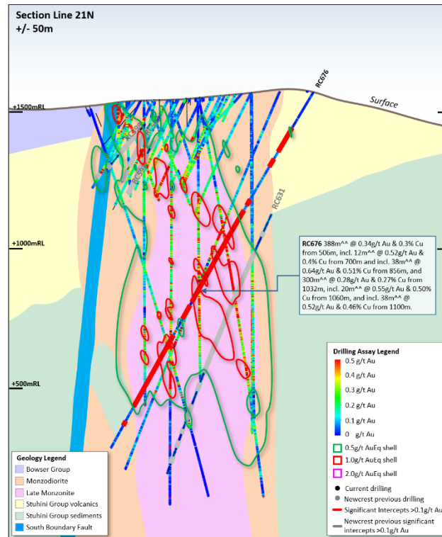
Figure 11. Schematic cross section of RC676 ( Section Line 21N ) showing Newcrest and Imperial drill holes and Newcrest intercepts (drill intercepts have been reported in Appendix 1 of this report, and in prior Newcrest exploration releases) 0.5 g/t AuEq, 1 g/t AuEq and 2 g/t AuEq shell projections generated from Leapfrog model. Due to window size (+/- 50m) and section orientation (150°) hole may appear on multiple sections.
