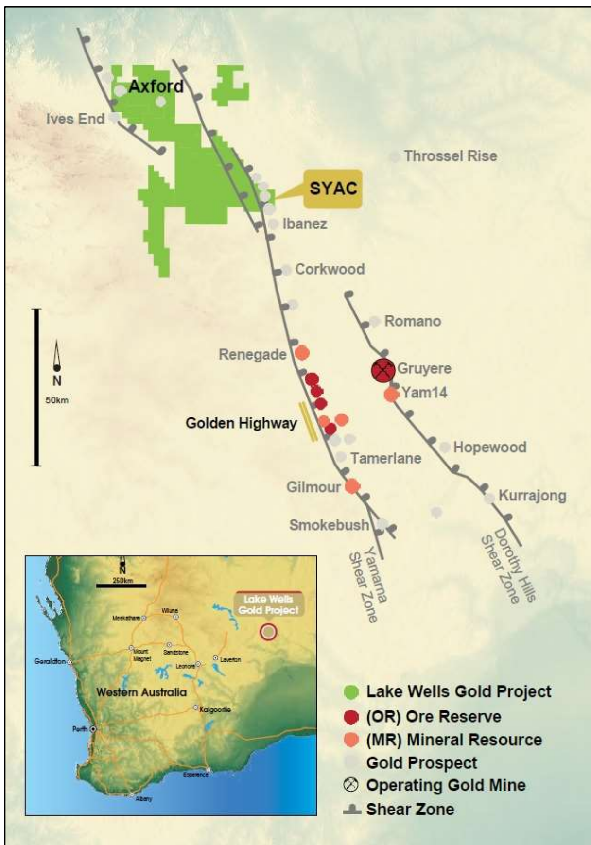
Figure 1: Location map for Lake Wells Gold JV, regional gold mineralisation and the South Yamarna Anomaly Camp (SYAC).
