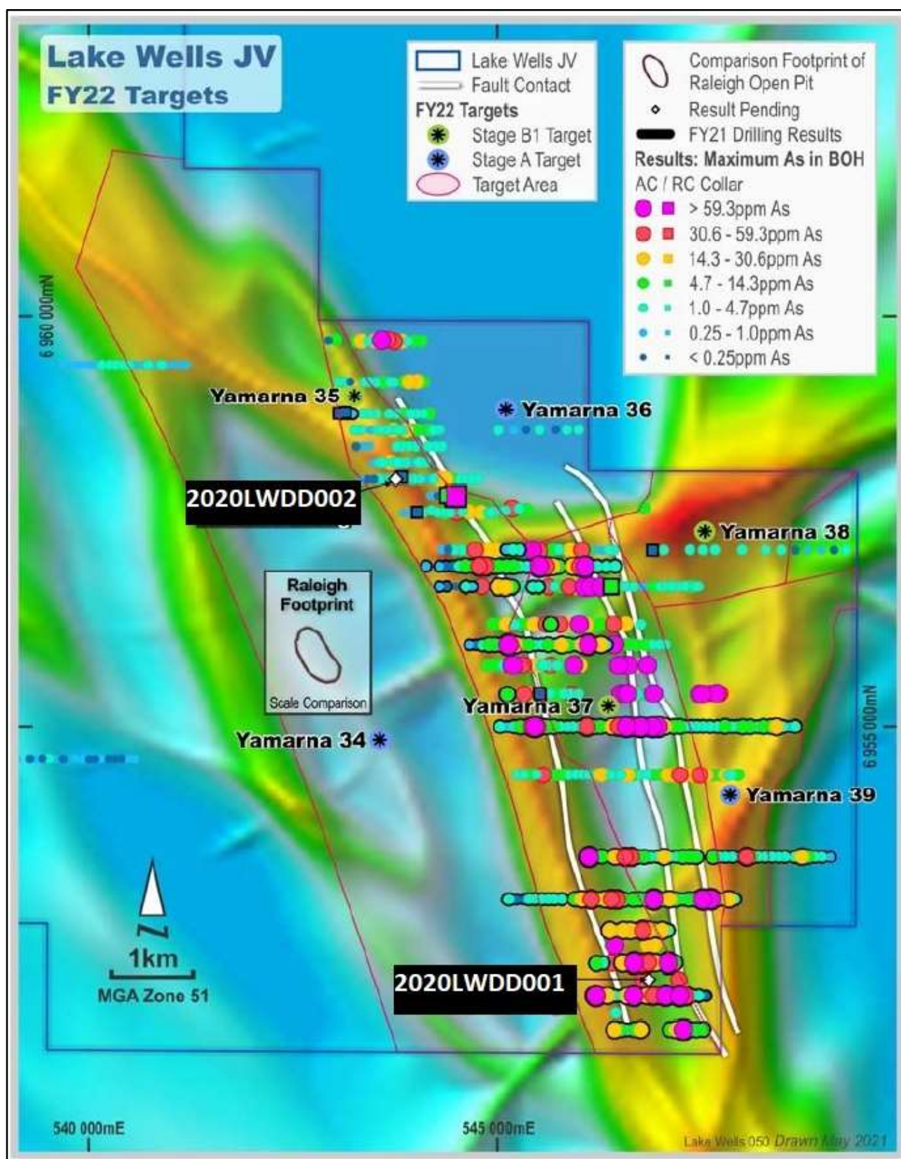
Figure 2: Exploration drill hole locations for the South Yamarna Anomaly Camp (SYAC) highlighting the elevated arsenic in bedrock and DD collar locations.
