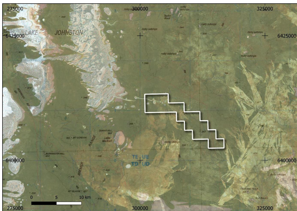
Figure 5:1 Taylors Rock Project – Location & Topography
