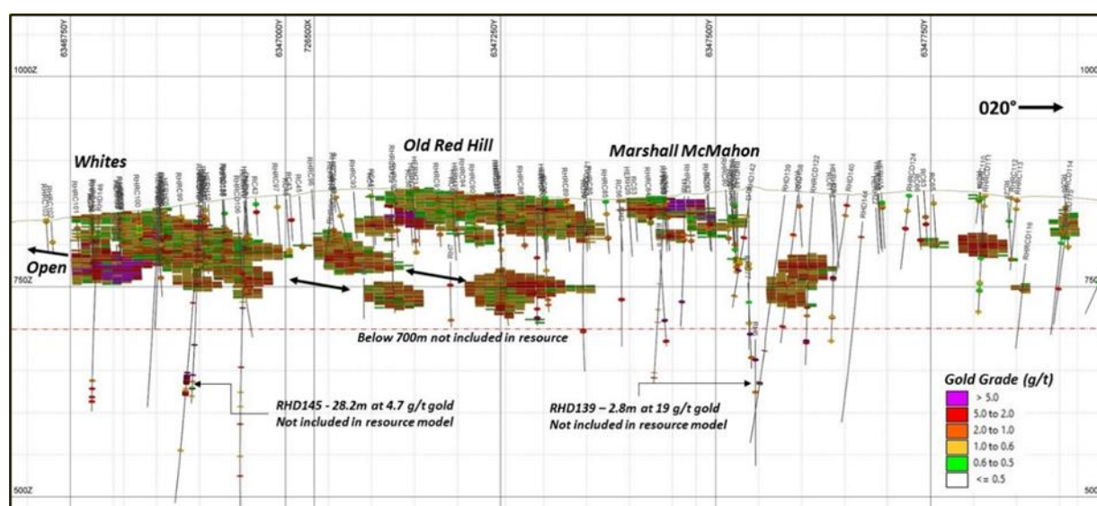
Figure 3:6 Red Hill Resource – Representative longitudinal section looking WNW
