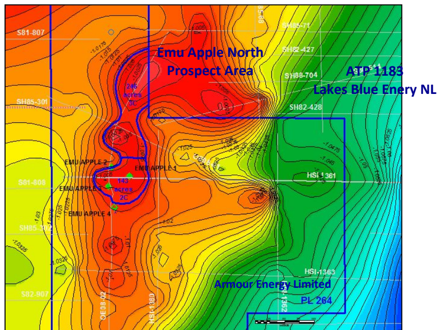
Figure 7: Emu Apple North Prospect
