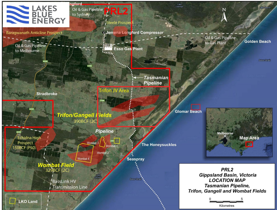
Figure 4: Location of Wombat and Trifon-Gangell Gas Fields
