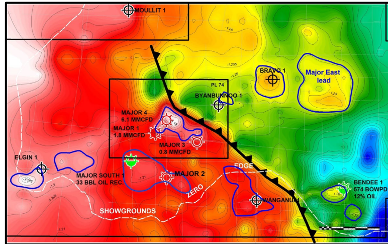
Figure 9: Major East Lead
