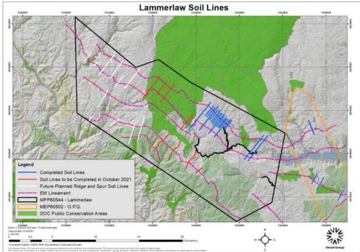
Figure 9: Planned Ridge and Spur Soil Lines at Lammerlaw
