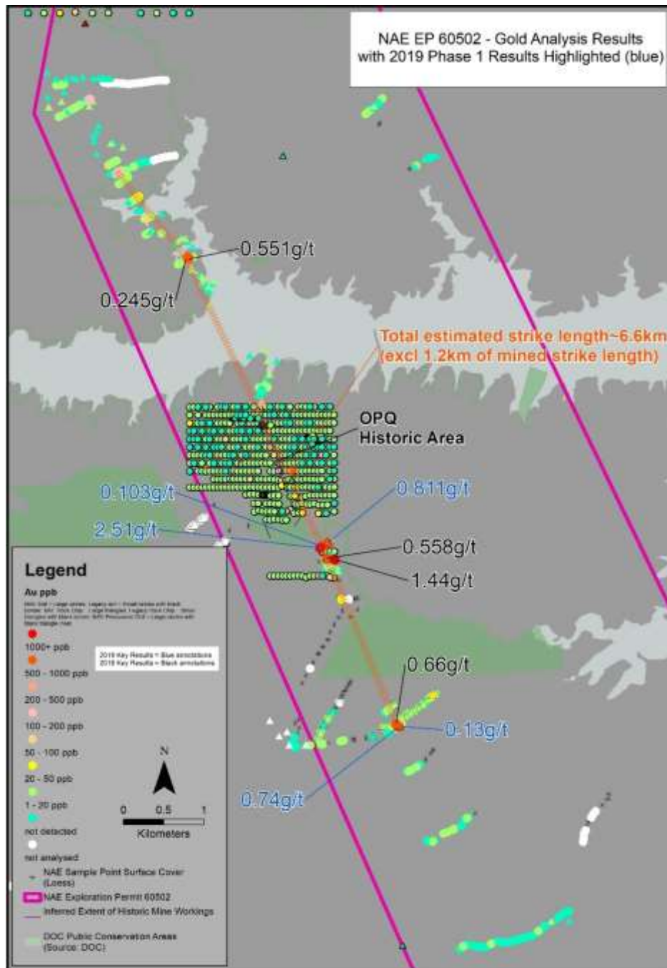
Figure 10: O.P.Q. estimated strike length. Taken from NAE ASX Announcement 12 December 2019
