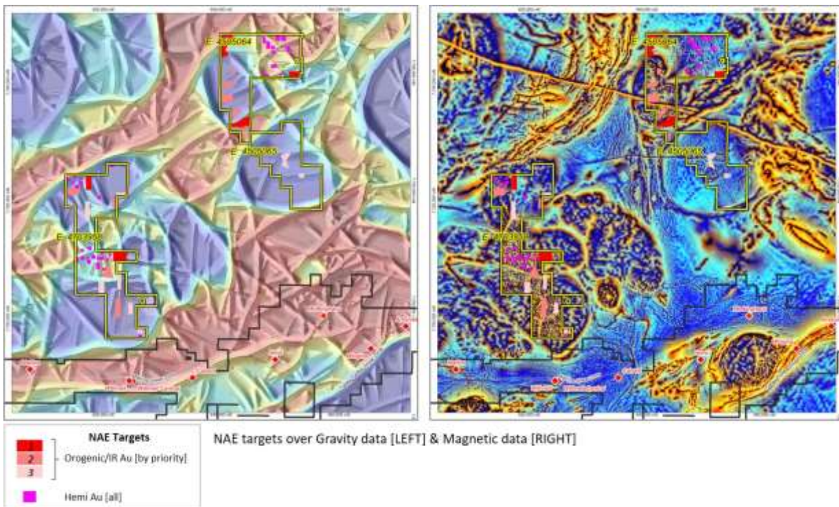
Figure 4: NAE targets over Bullock Well and Quartz Hill Gold Projects.
