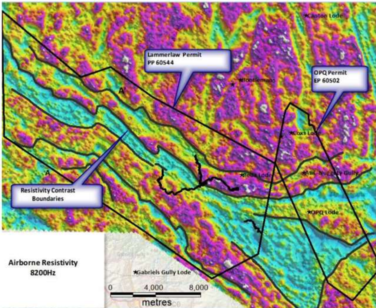
Figure 8: EM lineaments overlain by 8200Hz resistivity results
