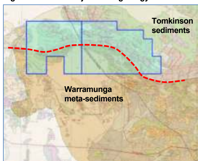
Figure 110 Duke Project local geology
