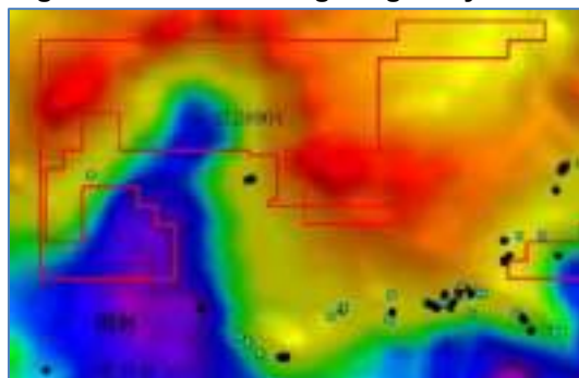
Figure 169 Manto Bouguer gravity
