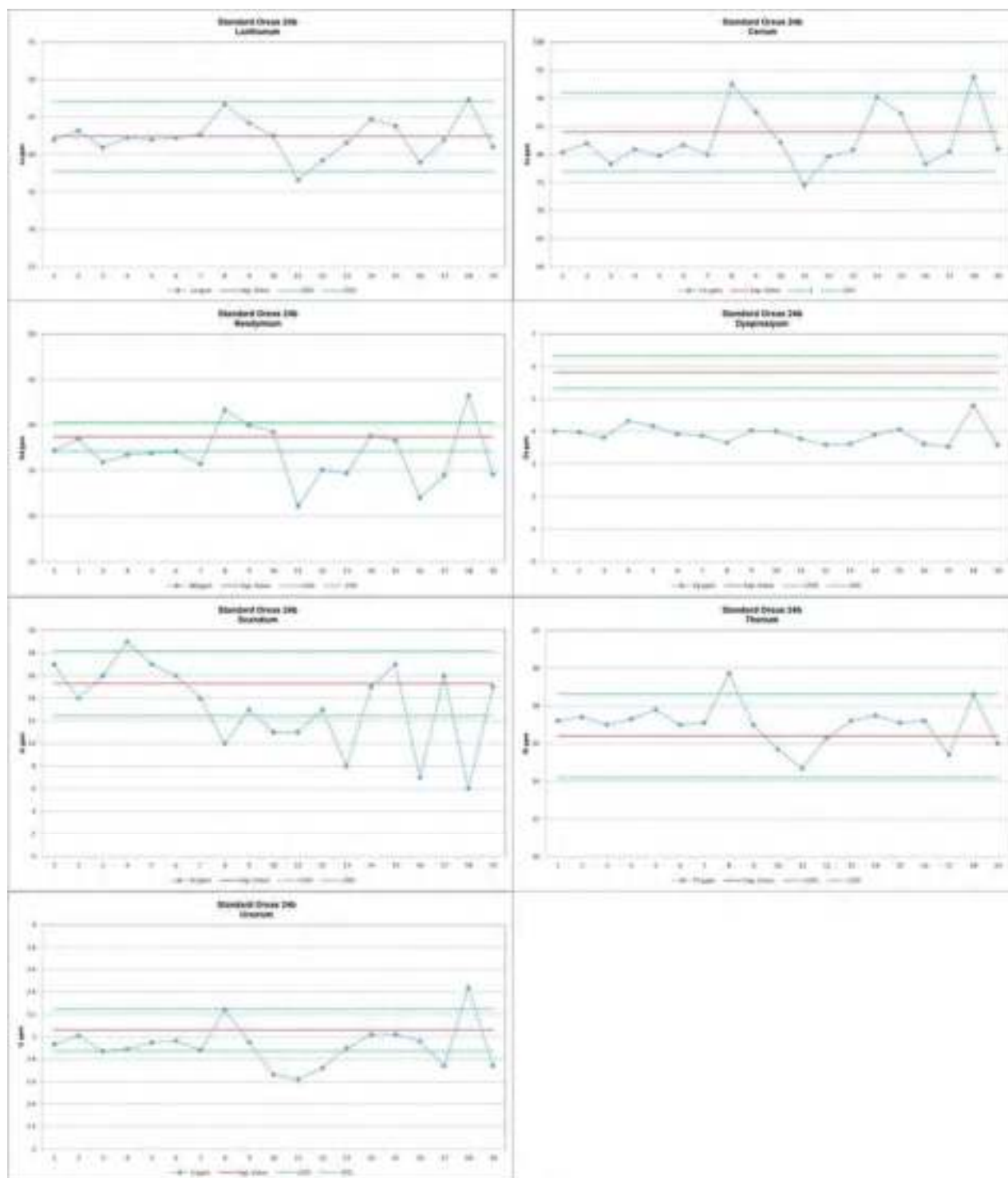
Figure 3-6 LabWest inserted standard OREAS 24b – La, Ce, Nd, Dy, Sc, Th & U
