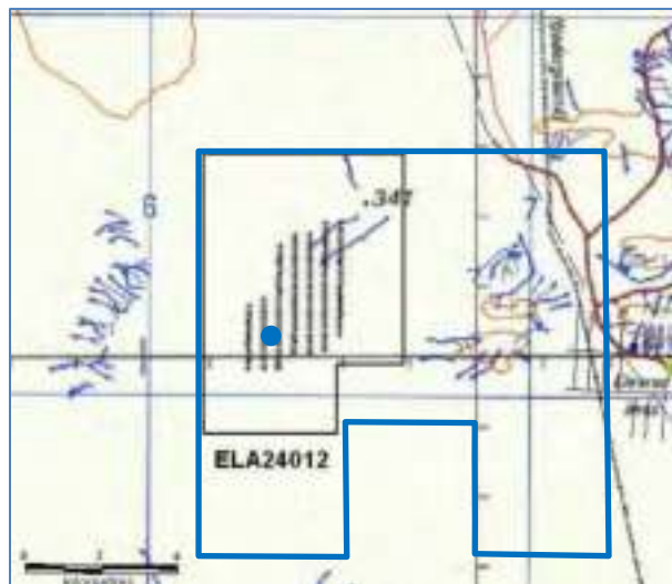
Figure 147 Red Metal EL24012 & gravity survey
