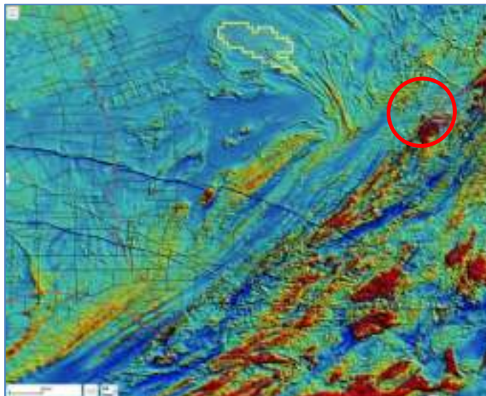
Figure 58 Salazar regional magnetics
