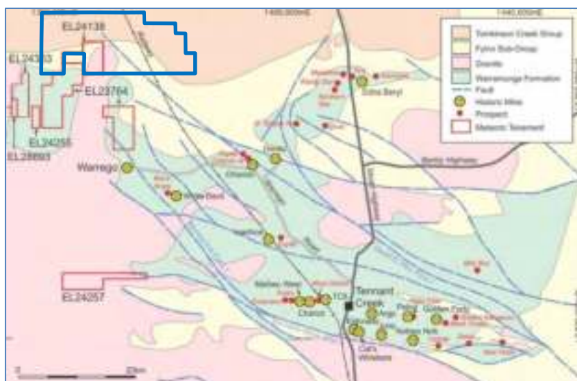
Figure 150 Meteoric's Tennant Creek Project geological setting
