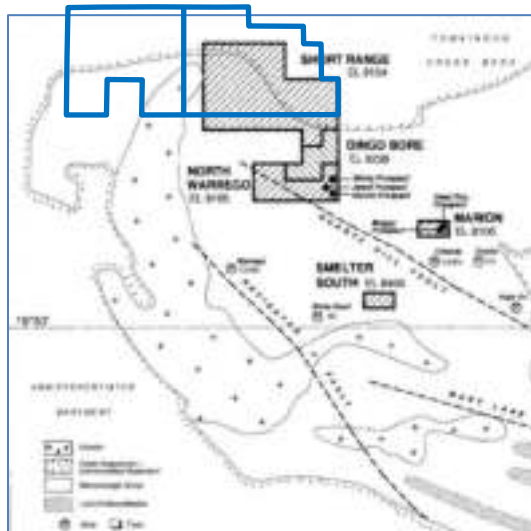
Figure 145 Delta Gold early prospects & Geochem areas
