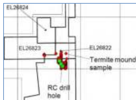
Figure 156 Sipa exploration 2009/10
