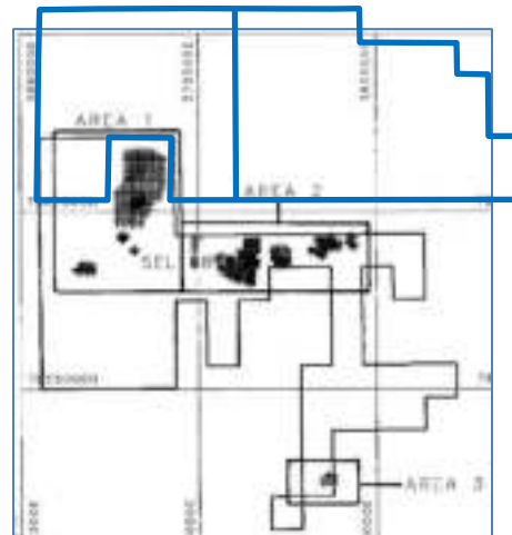
Figure 142 PosGold vacuum drilling
