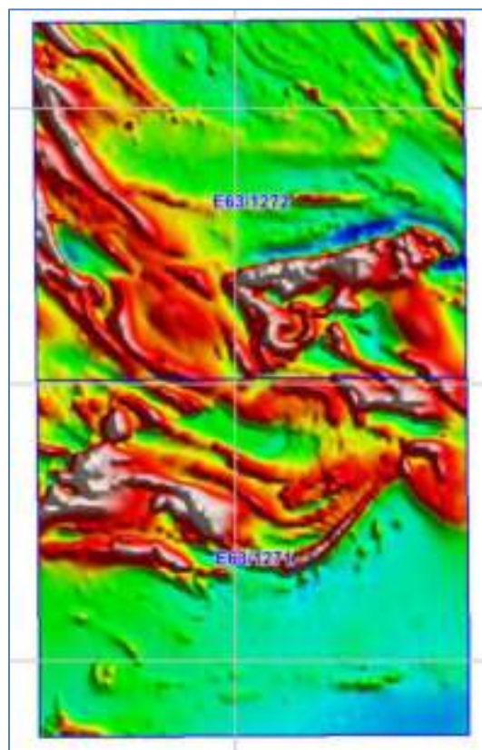
Figure 42 AngloGold TMI
