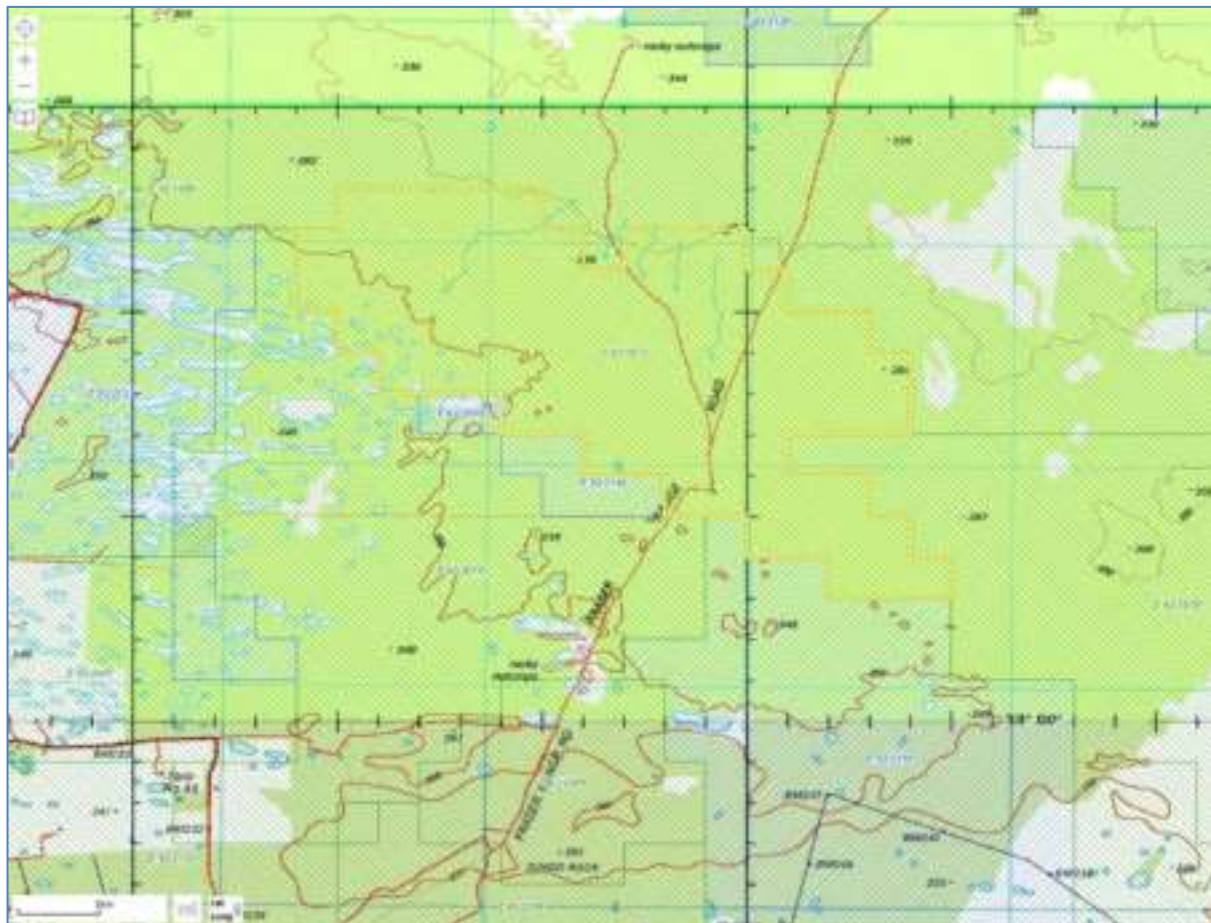
Figure 33 Adjacent tenements to E63/1972 at 10/1/2022
