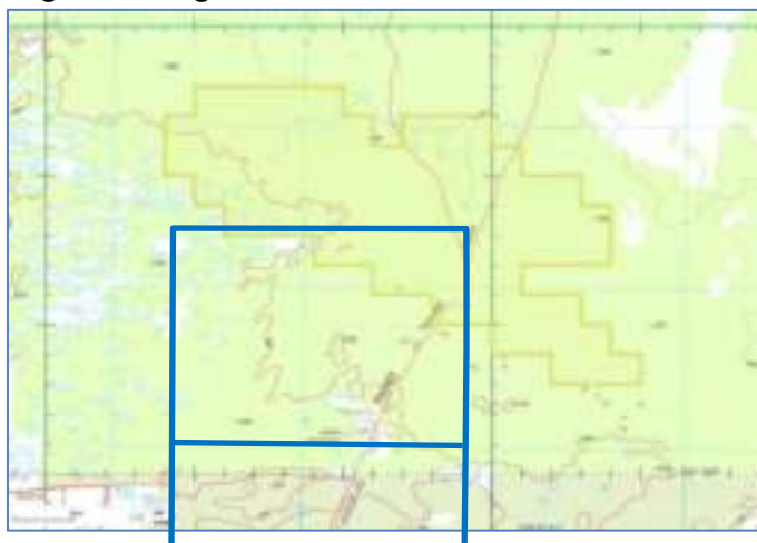
Figure 41 AngloGold's E63/1272
