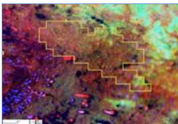
Figure 39 Radiometrics
