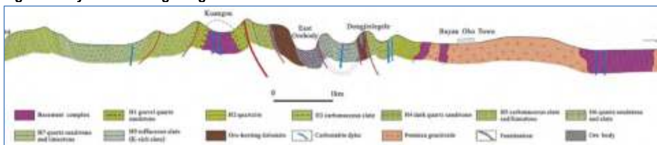
Figure 7 Bayan Obo N/S geological cross-section
