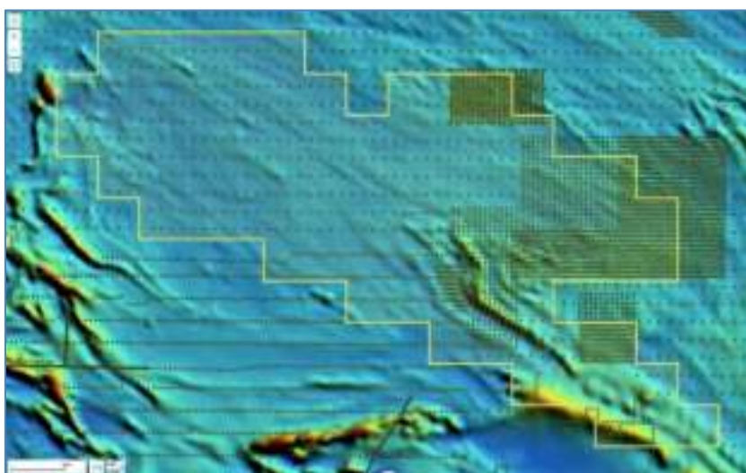
Figure 65 Surface sampling locations above magnetics
