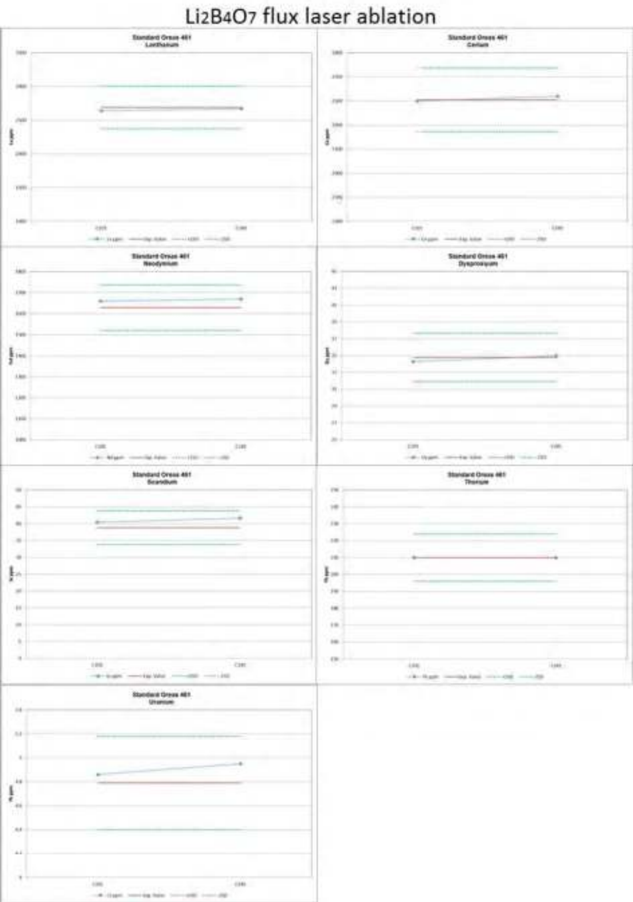
Figure 3-15 BV Pulp Checks; Standard OREAS 461 – La, Ce, Nd, Dy, Sc, Th & U
