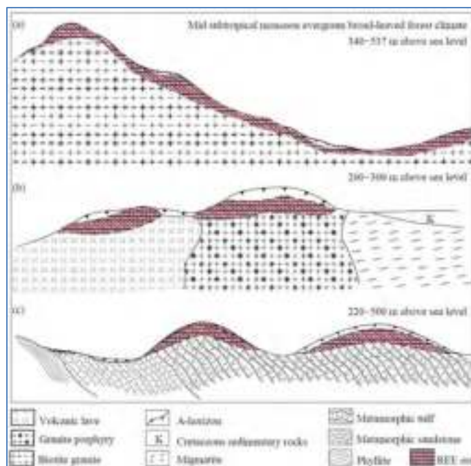
Figure 17 IAC deposits above different source rocks
