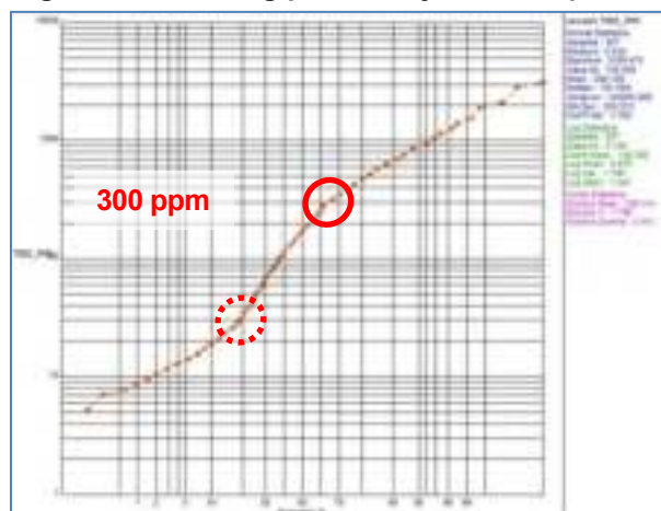
Figure 89 TREE log probability – all samples
