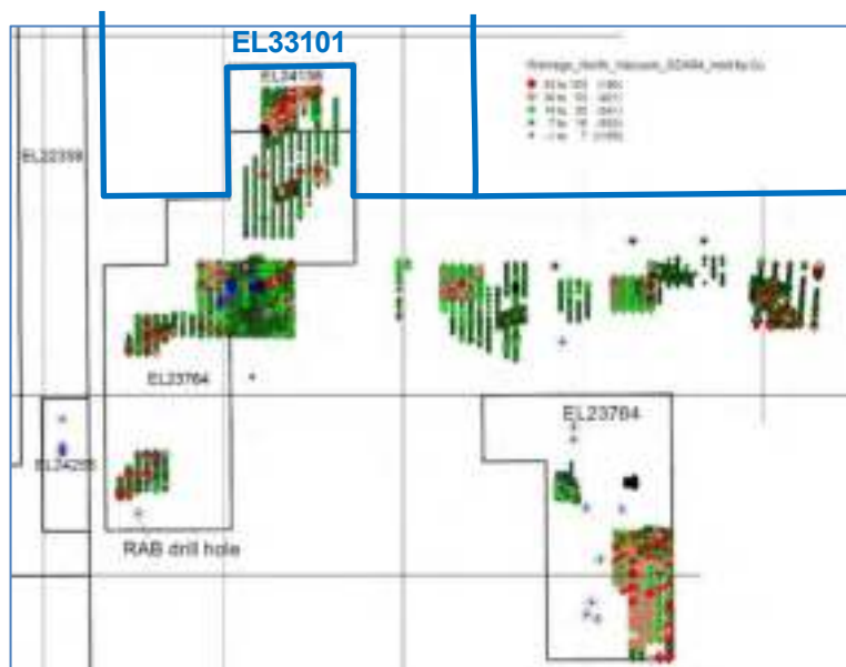
Figure 153 Vacuum drilling copper results
