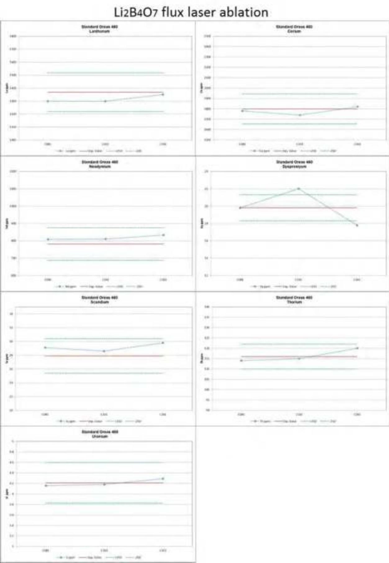
Figure 3-14 BV Pulp Checks; Standard OREAS 460 – La, Ce, Nd, Dy, Sc, Th & U
