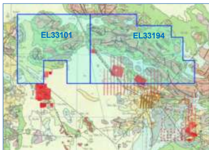
Figure 113 Duke Project past geochem sampling
