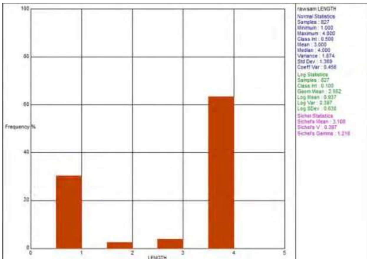
Figure 4-8 Normal histogram for length – All raw samples
