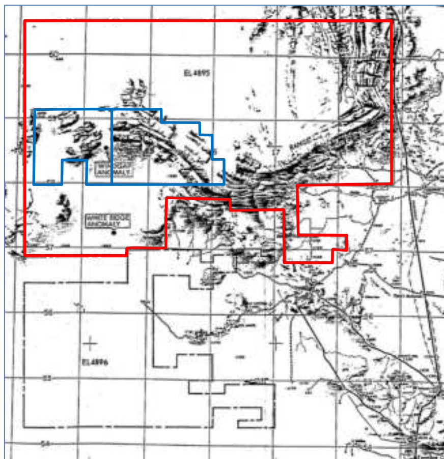
Figure 131 CEGBEA / Pos Gold EL4895 & EL4896
