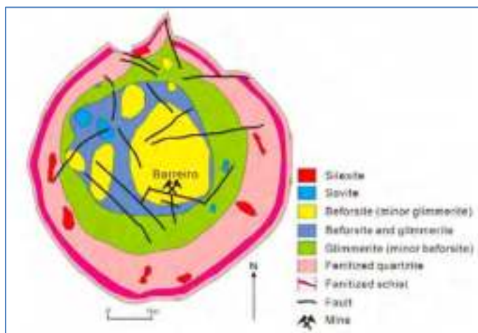
Figure 12 Araxá carbonatite geology plan
