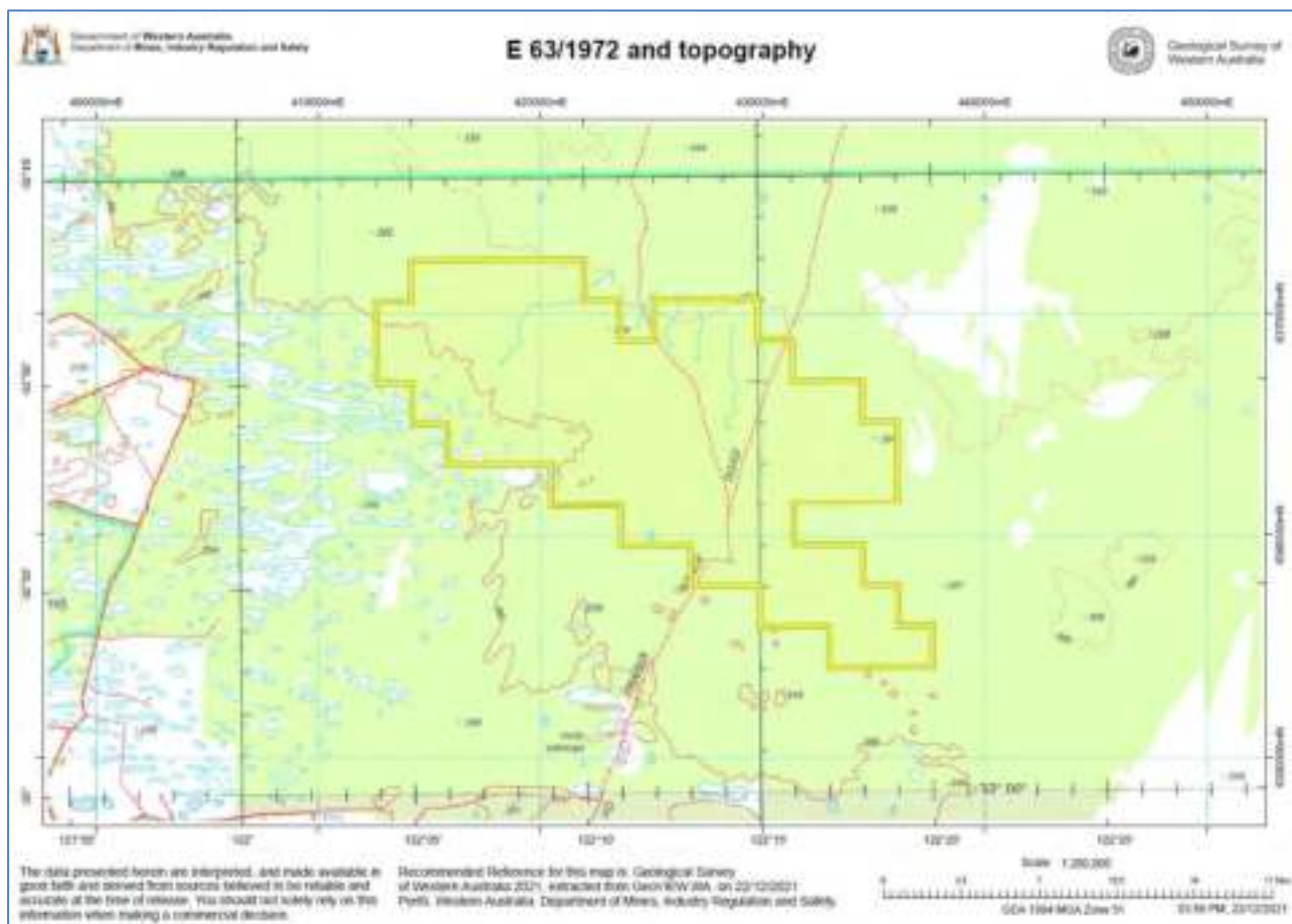
Figure 32 HRE Cowalinya Project tenement E63/1972
