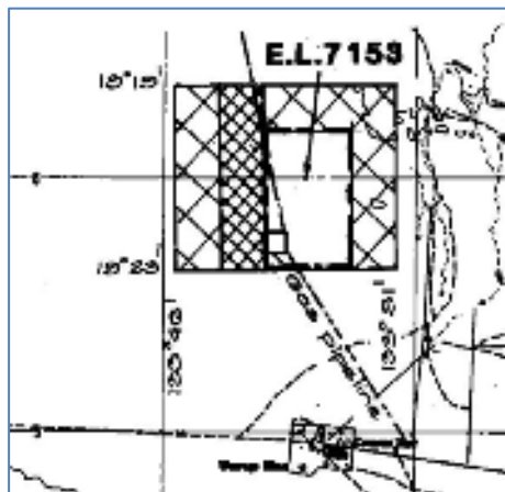
Figure 138 WMC EL7153 reductions
