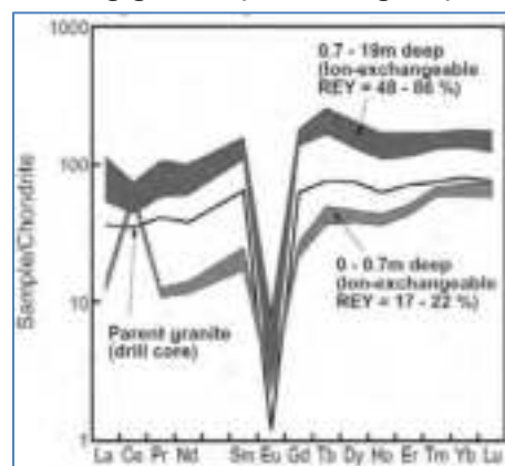
Figure 16 REE distribution in Zudong granite (below Lognan)
