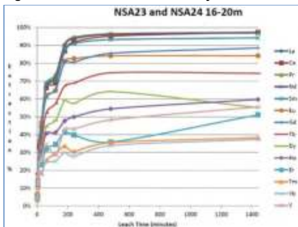
Figure 64 Individual REE recovery
