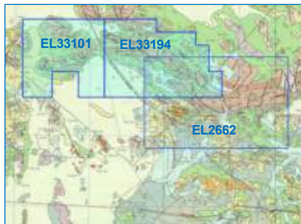
Figure 130 CRAE EL2662 (Last Hope)
