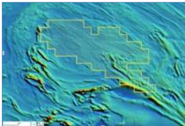
Figure 40 Magnetics
