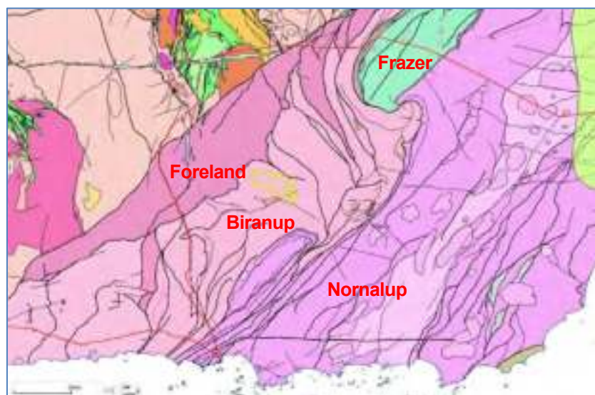
Figure 35 Regional bedrock geology
