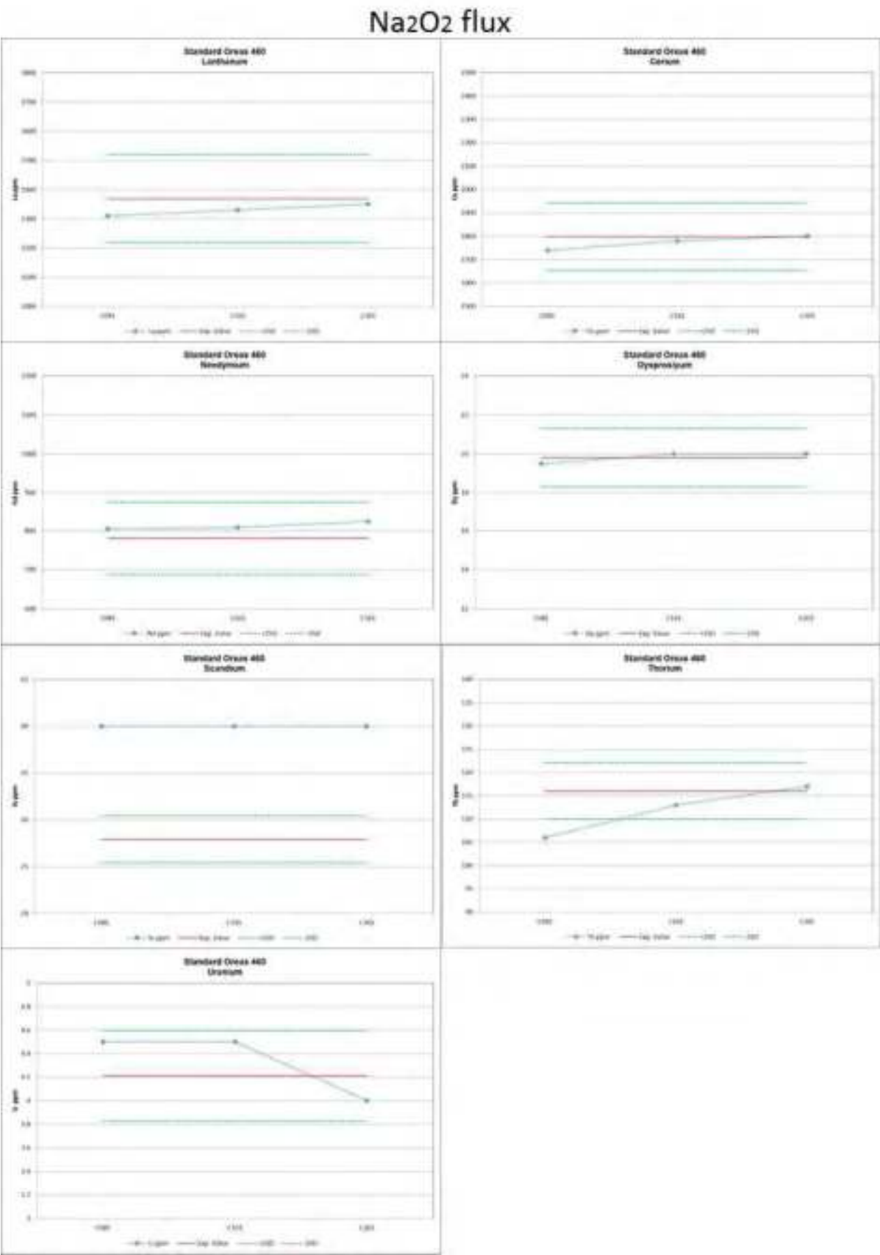
Figure 3-17 BV Pulp Checks; Standard OREAS 460 – La, Ce, Nd, Dy, Sc, Th & U
