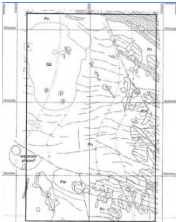
Figure 141 EL7896 photogeological interp
