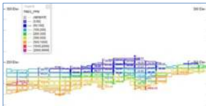
Figure 96 TREO block cross-section 6,361,000 N (North Area)
