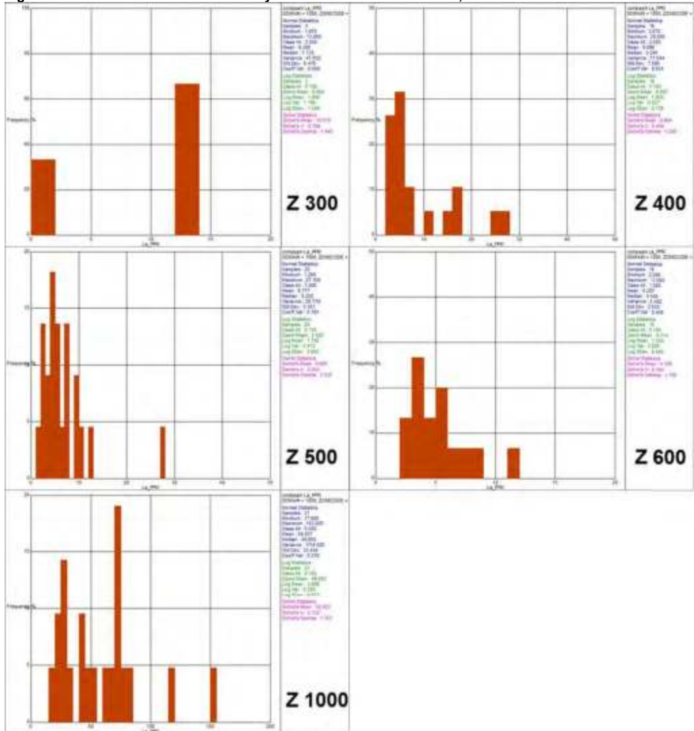
Figure D-3 Statistics Plots – Cowalinya North – Other ZONECODEs; La
