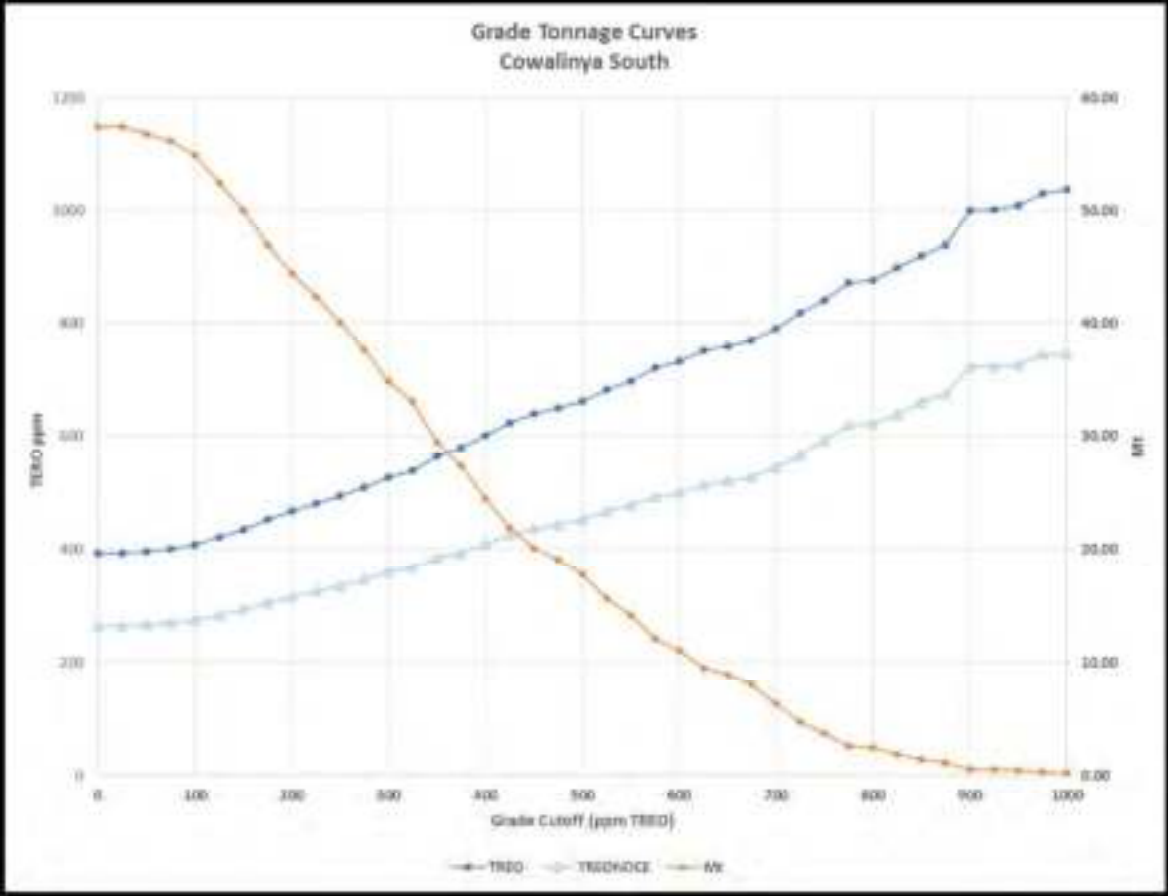
Figure 5-2 Grade Tonnage curves, Cowalinya South
