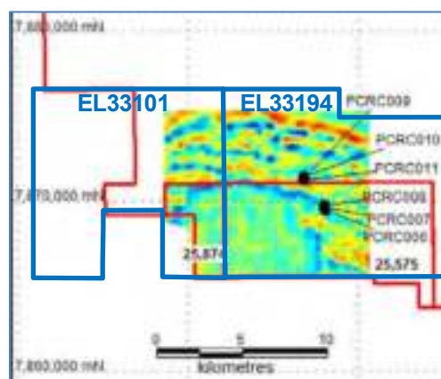
Figure 160 Uranium West magnetics
