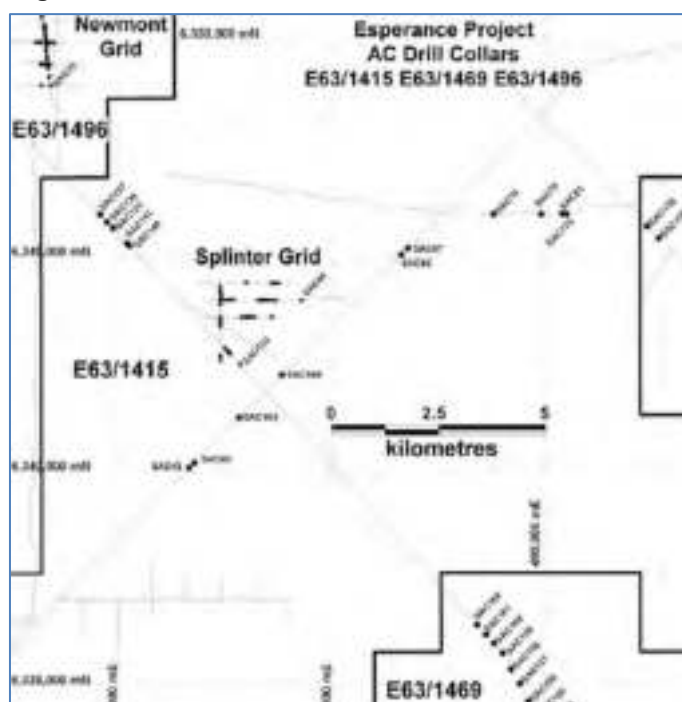
Figure 61 Salazar drill hole locations
