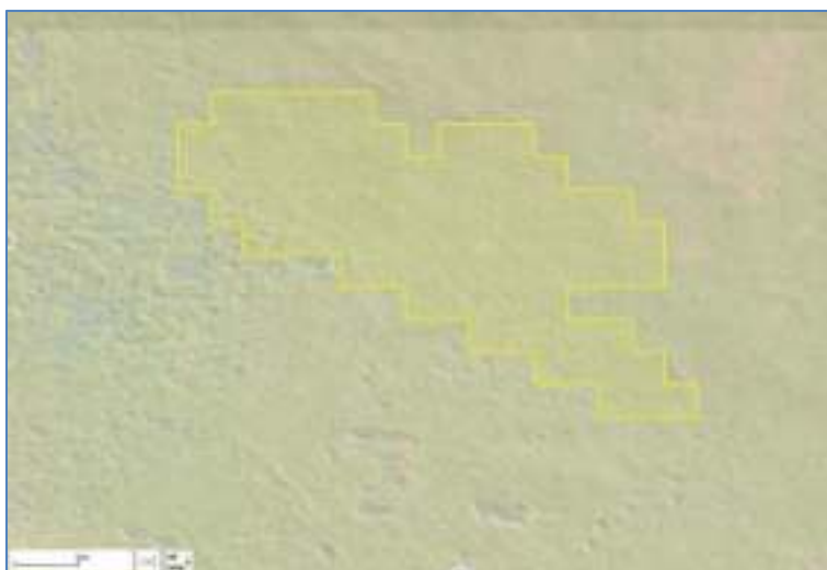
Figure 31 Cowalinya STRM3 slope topography
