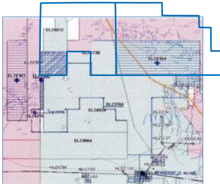
Figure 148 Meteoric ELs in Warrego North & West Projects
