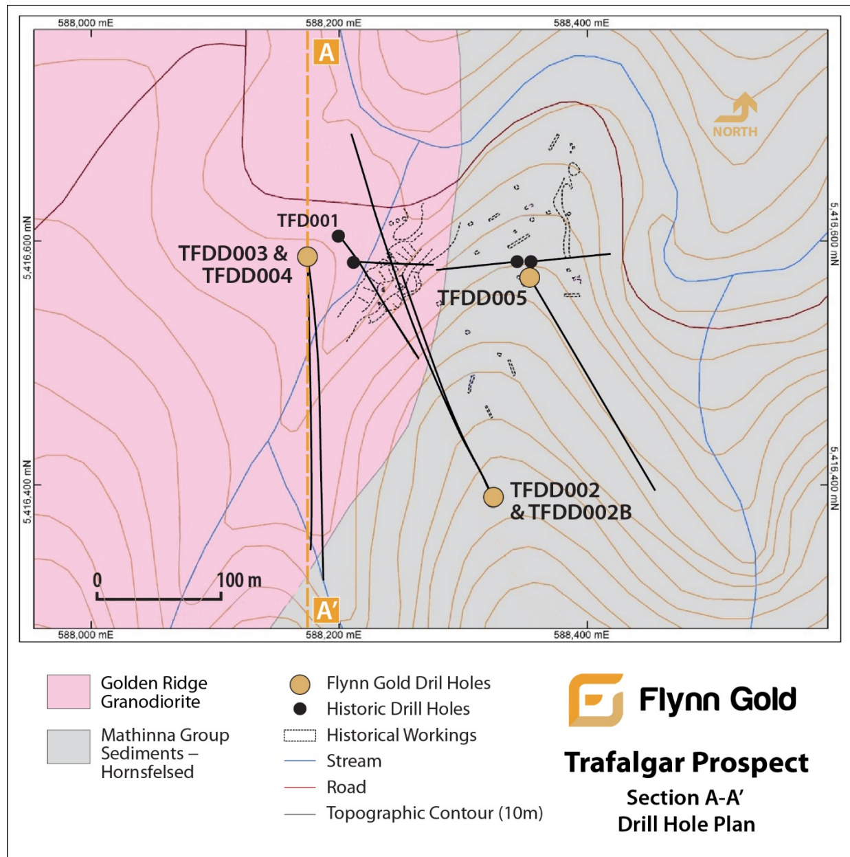
Figure 2: Trafalgar Prospect Drill Hole Plan.
