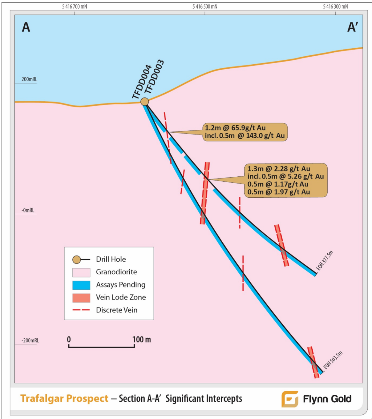
Figure 3: Cross-section showing drill holes TFDD003 and TFDD004.
