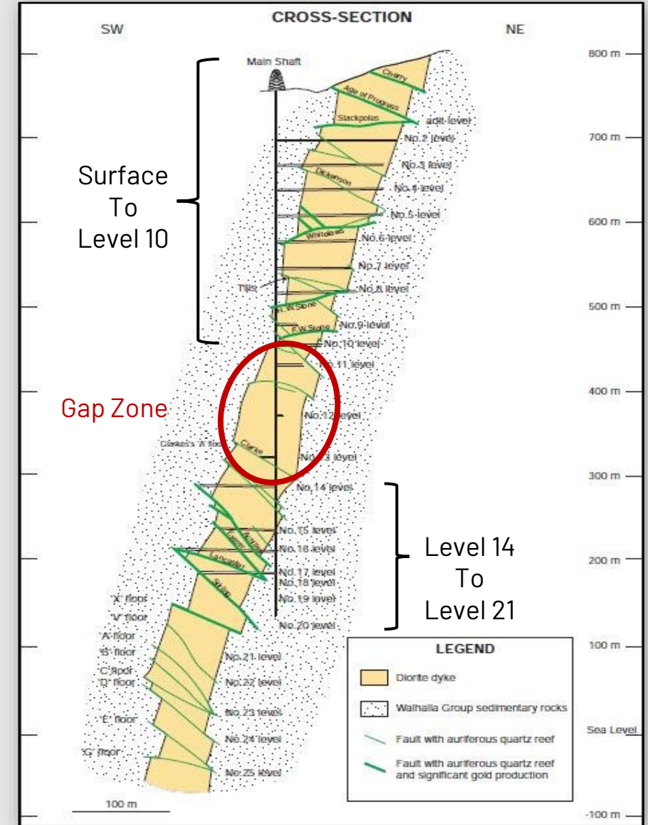
Cross-section of the Morning Star gold mine showing west and east-dipping mineralised faults that transect a diorite dyke, highlighting the prospective Gap Zone.
