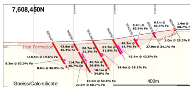
Figure 6: Southern Zone cross Section 7,608,450N. High-grade ~60% Fe and ~61% Fe at surface in BEKD 18 and BEKD 55 and at depth a continuous 150.8 metres iron intercept at 33.2% Fe in BEKD 59.
