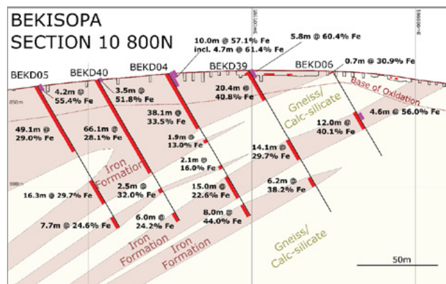
Figure 5: Central Zone cross section along latitude 7610800 incorporating Bekisopa drill holes. BEKD 04, BEKD 05 and BEKD 06 from the 2020 drilling programme and drill holes. BEKD 39 and BEKD 40 from the 2021 drilling campaign
