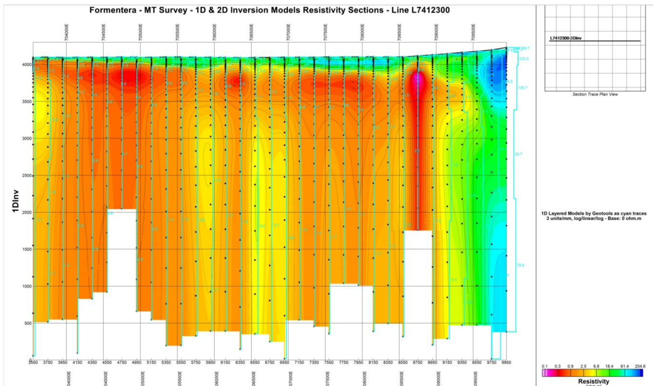
Figure 5. Line 2300 1D inversion shows an extremely low resistivity unit of 0.1ohm-m to the east (area in pink and red) and several areas between 3500m and 4000m in red that shows possibly a 300-400m thick aquifer.
