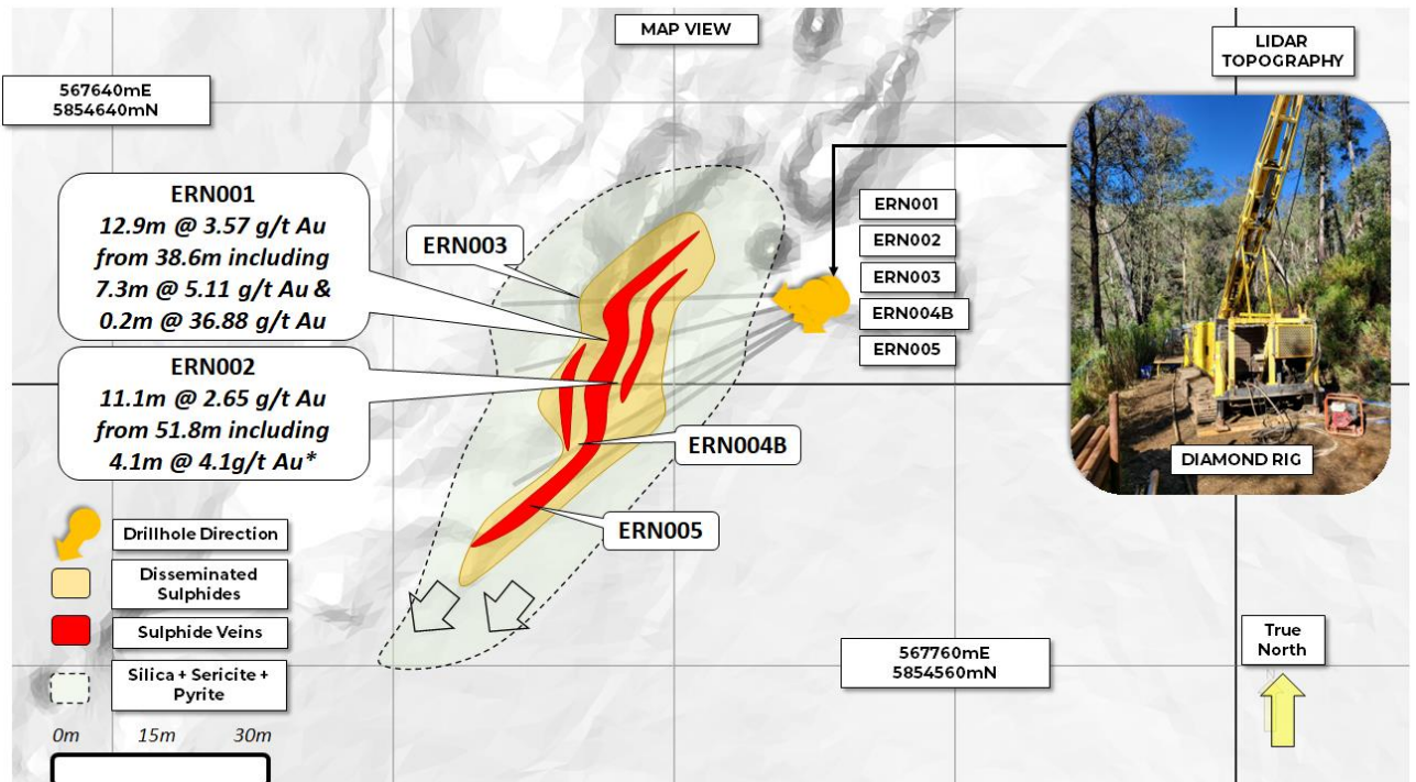
Figure 2: Plan view of drilling completed to date with assay results ERN0001 & ERN0002, over LIDAR topography. All coordinates in MGA94 Zone 55.
