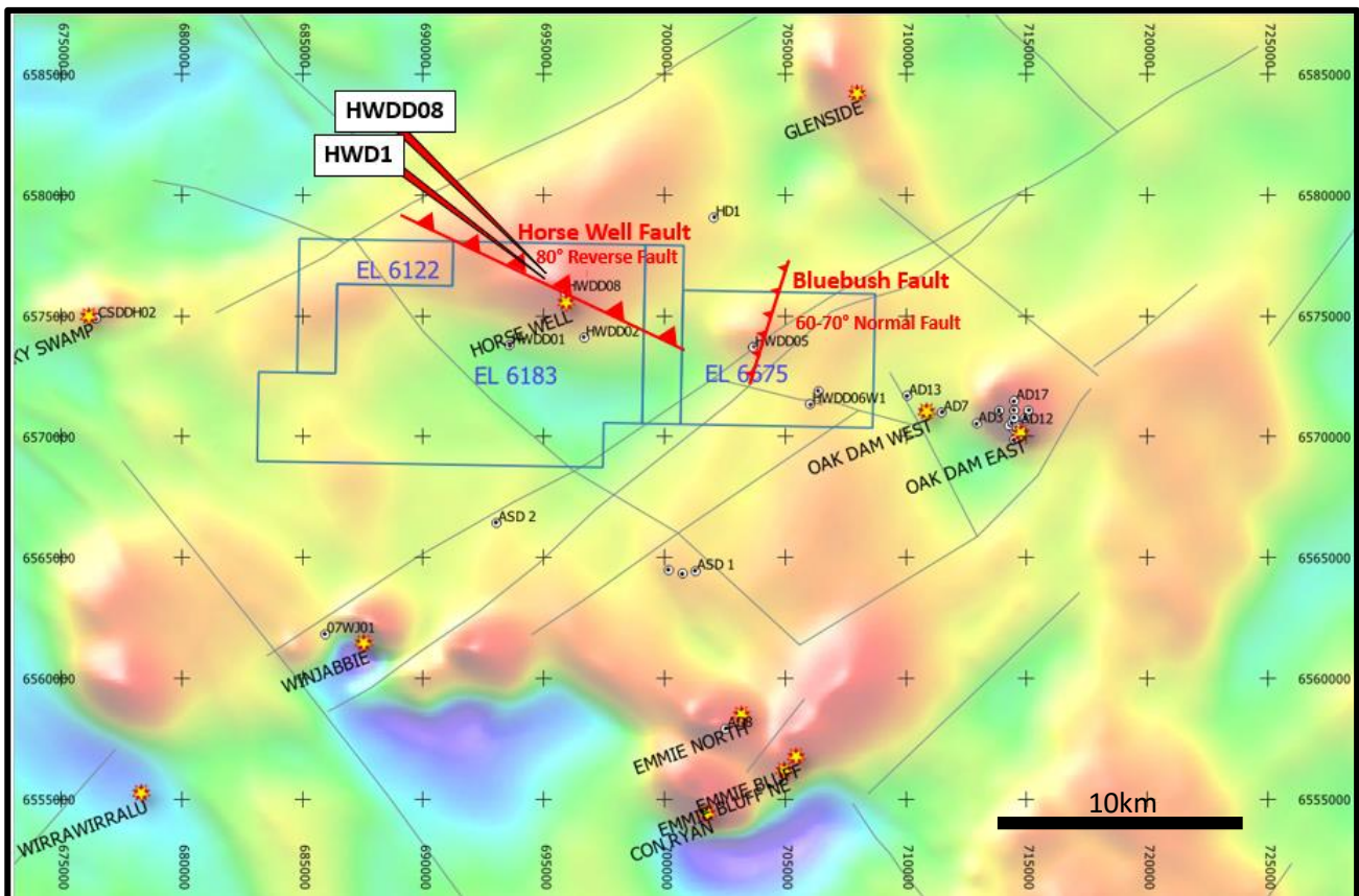
Figure 3: Regional Total Magnetic Intensity Map (TMI) with SARIG “Archaean – Early Mesoproterozoic faults’ interpreted lineaments, and the Horse Well Fault and HWDD08.
