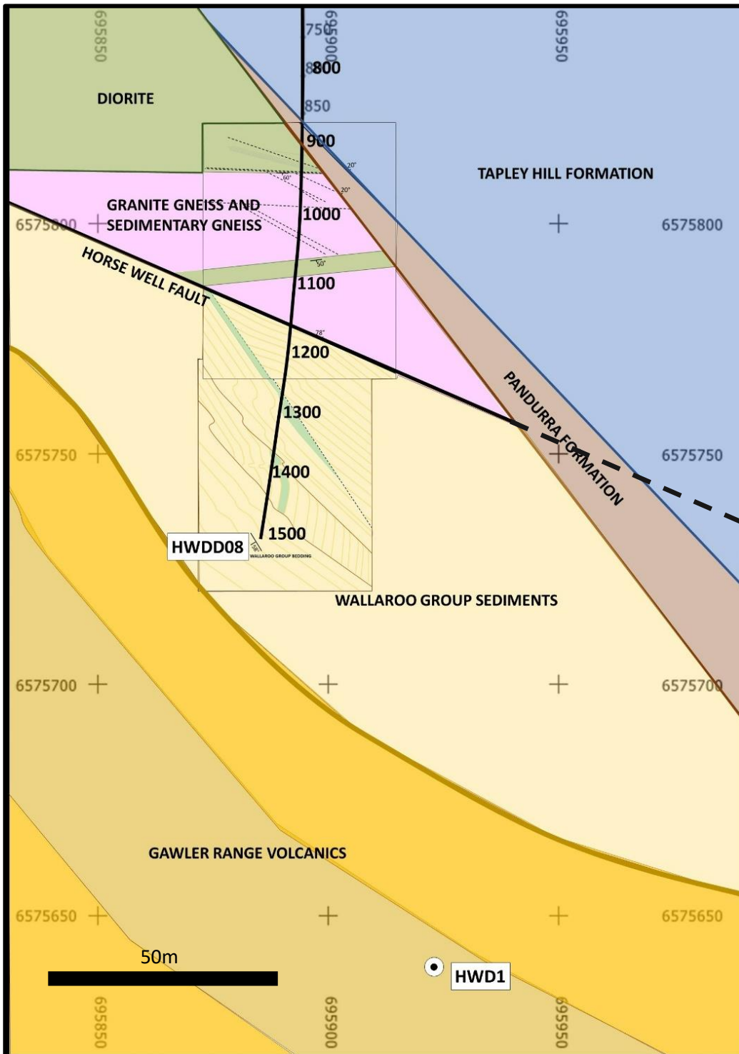
Figure 5: Horse Well Prospect pseudo plan-view looking down drill hole HWDD08.
