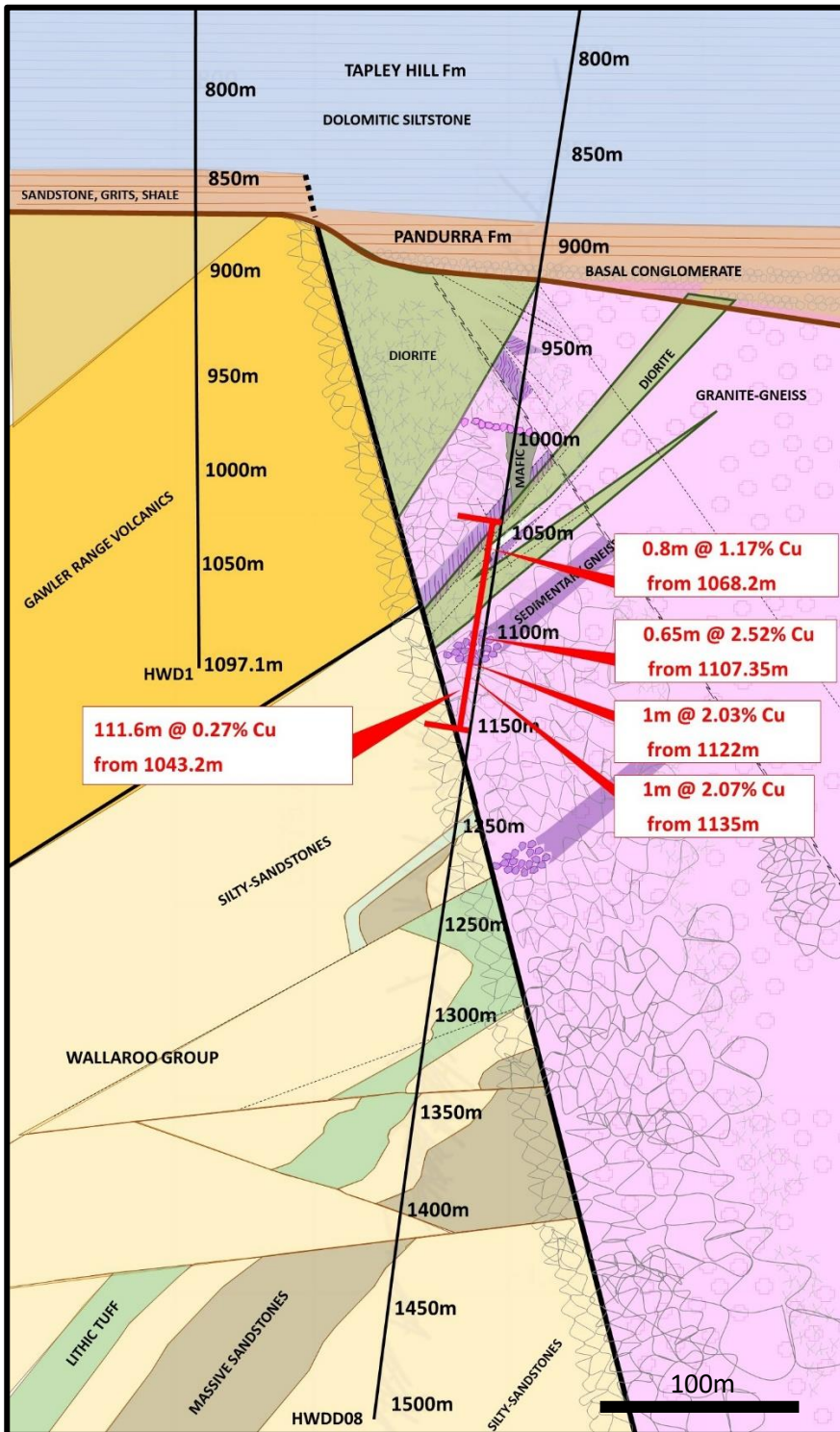
Figure 2: Interpreted Cross-Section HWDD08 and HWD1 looking west.
