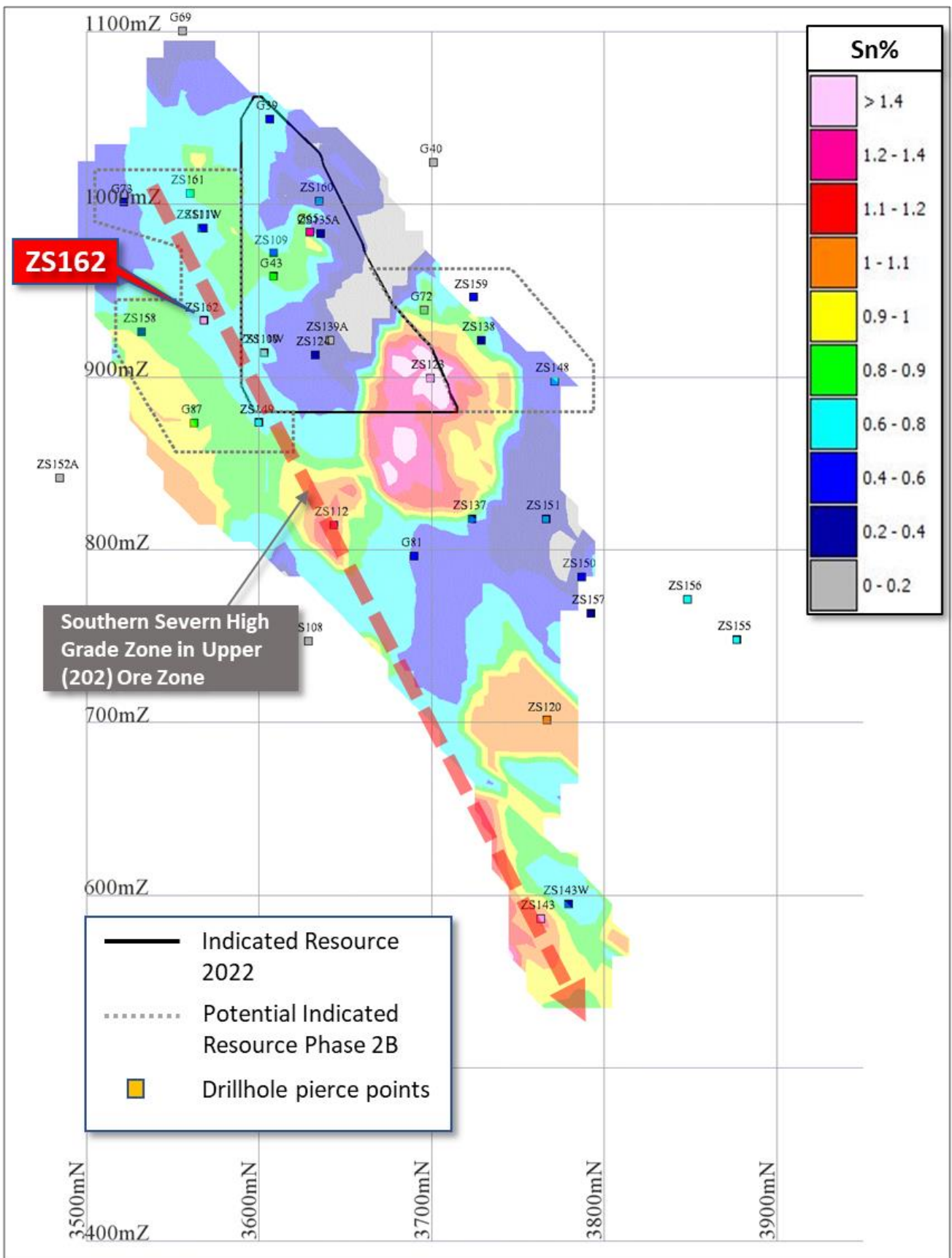
Figure 1 – Severn Upper (202) Ore Zone Long Section looking west showing Phase 2B and historic drillholes, Severn Resource and drillhole pierce points coloured by Sn% from Nov '22 Mineral Resource model (Zeehan Mine Grid)
