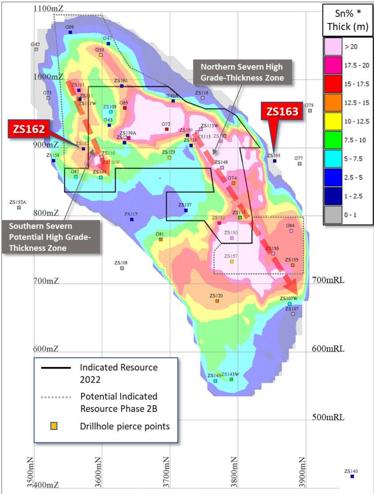
Figure 2 – Severn Main (201) Ore Zone Long Section looking west showing Phase 2B and historic drillholes, Severn Resource and drillhole pierce points coloured by Sn%*m from Nov '22 Mineral Resource model (Zeehan Mine Grid)
