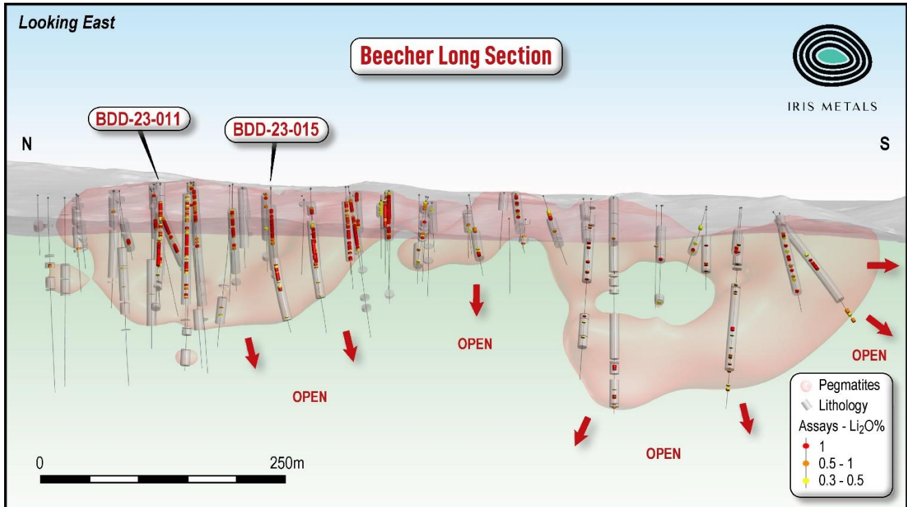
Figure 2: Long section looking east. Mineralisation remains open at depth and along strike to the south.
