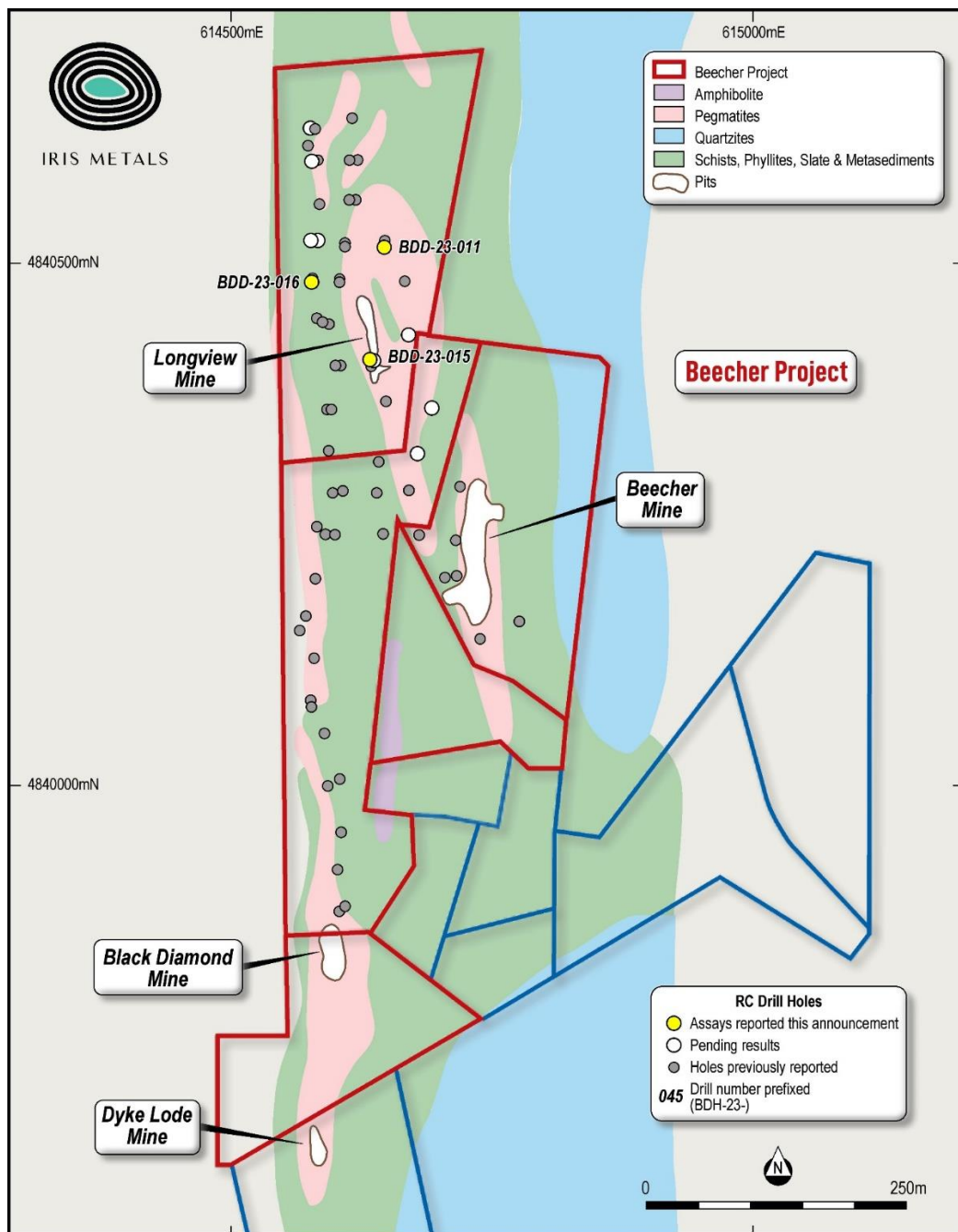
Figure 1: RC and diamond drill hole locations.
