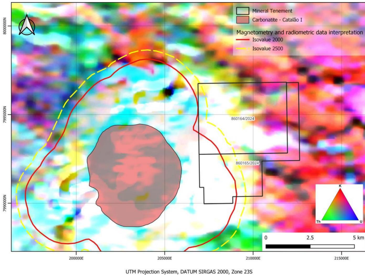
Figure 2. The interpreted magnetometry and radiometric data shows the high potential areas in white and the proximity to the Catalão carbonatite deposit. The isovalues 2000 represent the heat intensity from the contact metamorphism depositing the rare earths from fluids.
