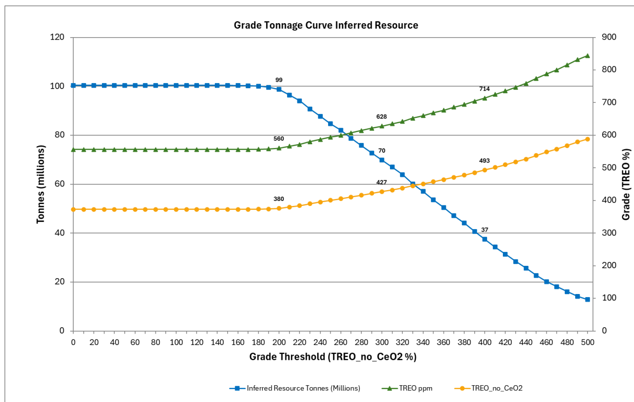
Figure 4: Grade Tonnage Curve – Inferred Resource.
