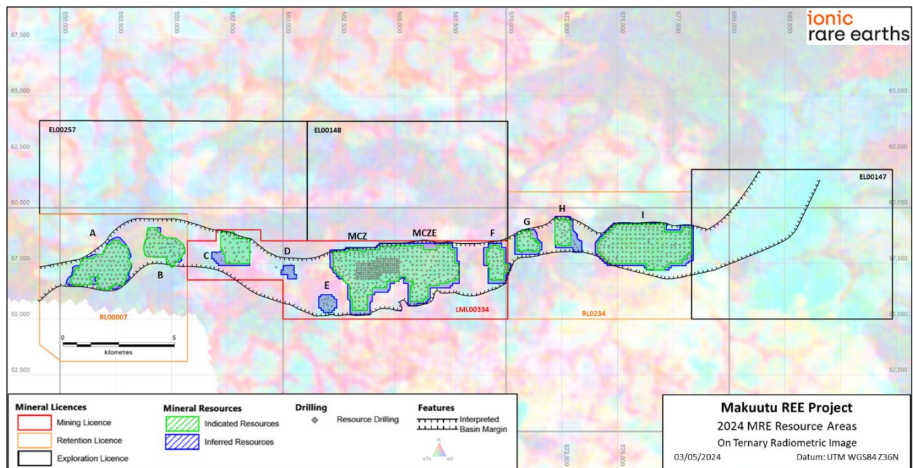
Figure 2: Plan view of MRE areas by classification. Green shading on Indicated resource areas and blue on Inferred resource areas with drill hole locations and mineral licences on ternary radiometric image.
