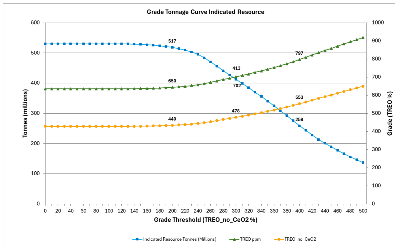
Figure 3: Grade Tonnage Curve – Indicated Resource.
