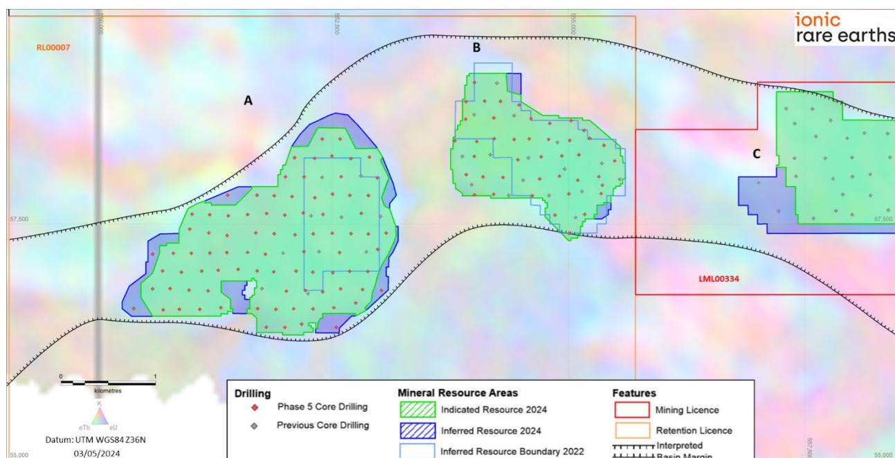
Figure 1: Resource areas A, B and C showing location of Phase 5 core drilling program (red points), previous drilling (grey points) with 2024 MRE Indicated Resource (green shade) and Inferred Resource (blue shade) and 2022 MRE inferred outline (pale blue).
