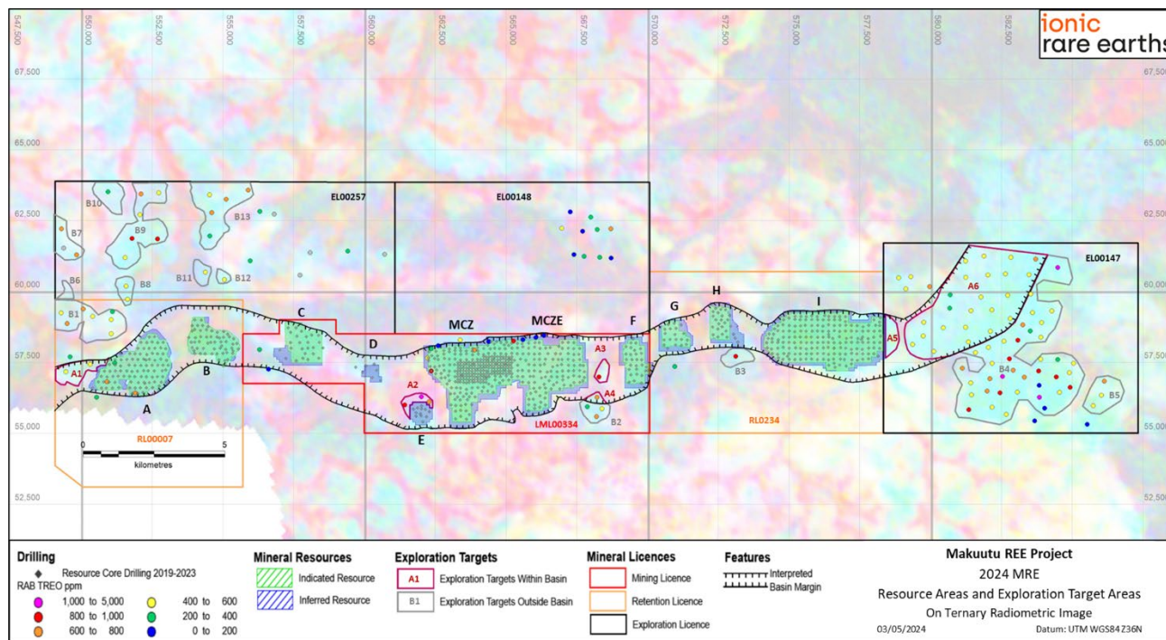
Figure 6: Makuutu project showing location of Exploration Target and Mineral Resource Areas.
