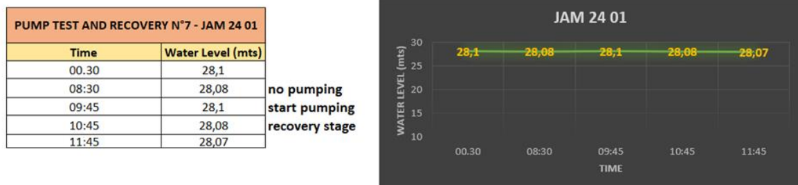
Figure 1. Water level in well Jam 24-01 not moving as pump test in Jam 24-02 takes place 300m away.
