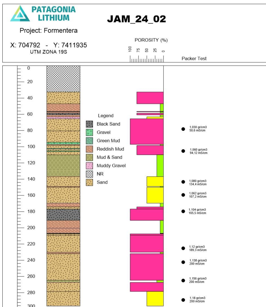
Figure 5. Lithological section showing porous sands and packer tests recording Specific gravity and conductivity.
