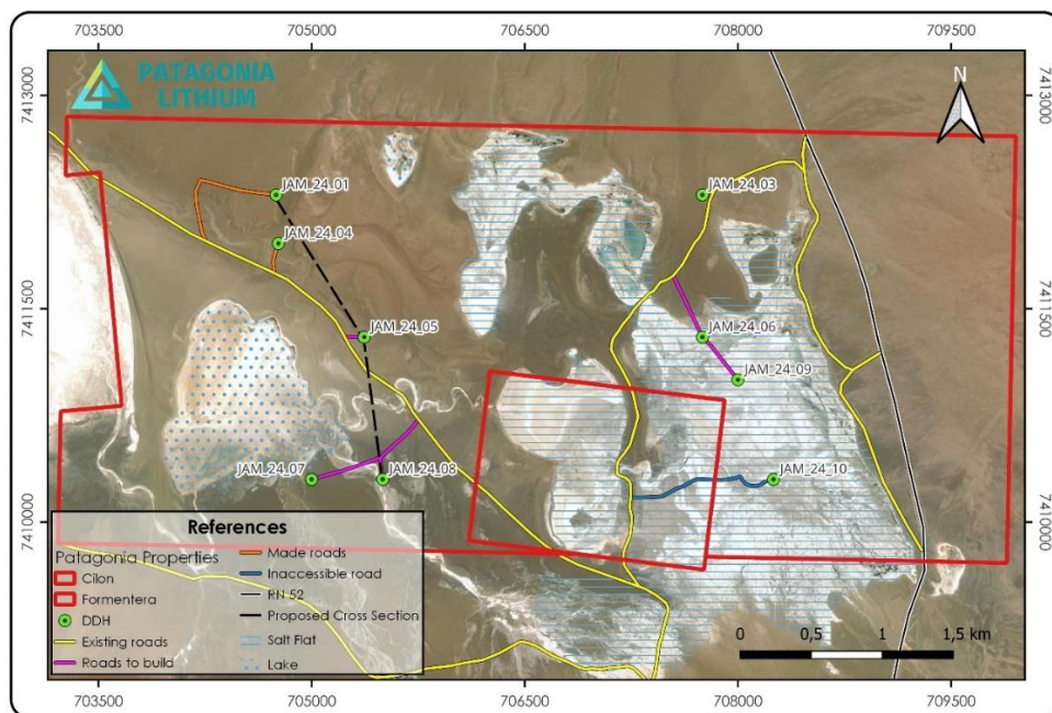
Figure 4. Map location of well two - labelled JAM 24-04, JAM 24-08 is next well to be drilled
