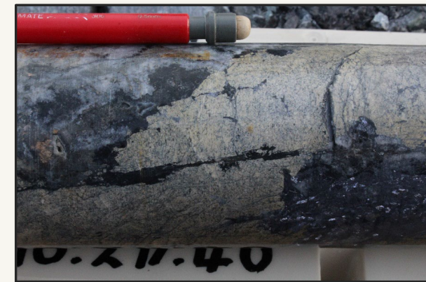
258.5m – White sphalerite and galena cut by MnO after rhodochrosite. 1m @ 654g/t Ag, 0.35g/t Au, +20% Pb, +30% Zn
