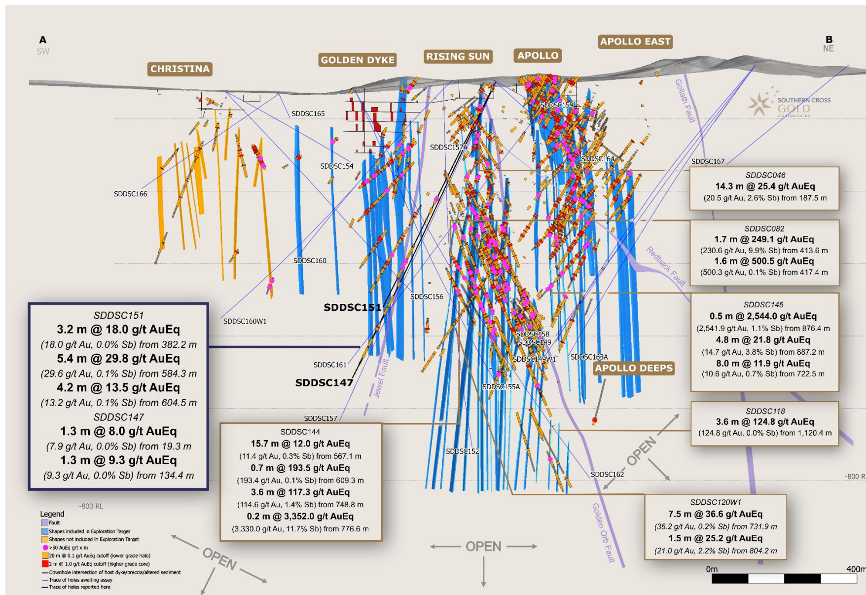
Figure 2: Sunday Creek longitudinal section across A-B in the plane of the dyke breccia/alterated sediment host looking towards the north (striking 236 degrees) showing mineralized veins sets. Showing holes SDDSC147 and SDDSC151 reported here (blue highlighted box, black trace), with selected intersections and prior reported drill holes. The vertical extents of the vein sets are limited by proximity to drill hole pierce points. For location refer to Figure 1.
