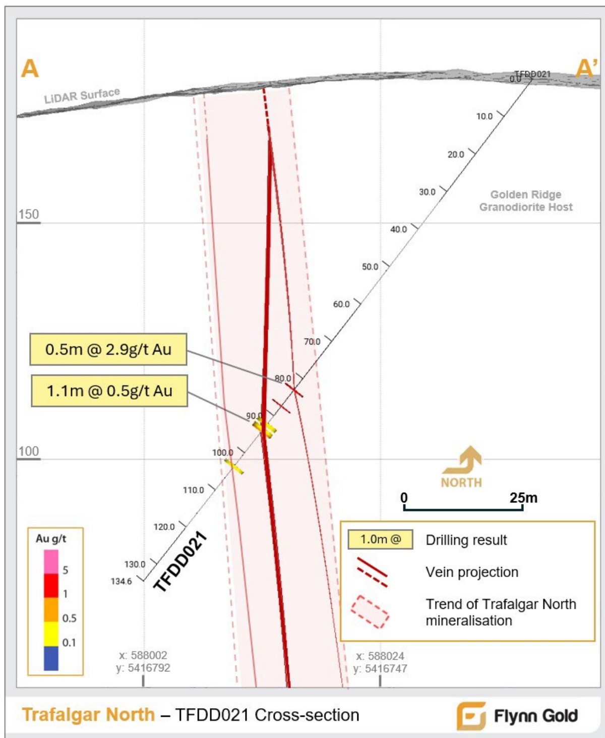
Figure 8 – Trafalgar North Prospect: TFDD021 Cross Section
