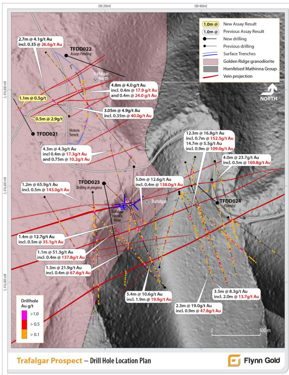
Figure 7 – Trafalgar Prospect: Drill Hole Location Plan.
