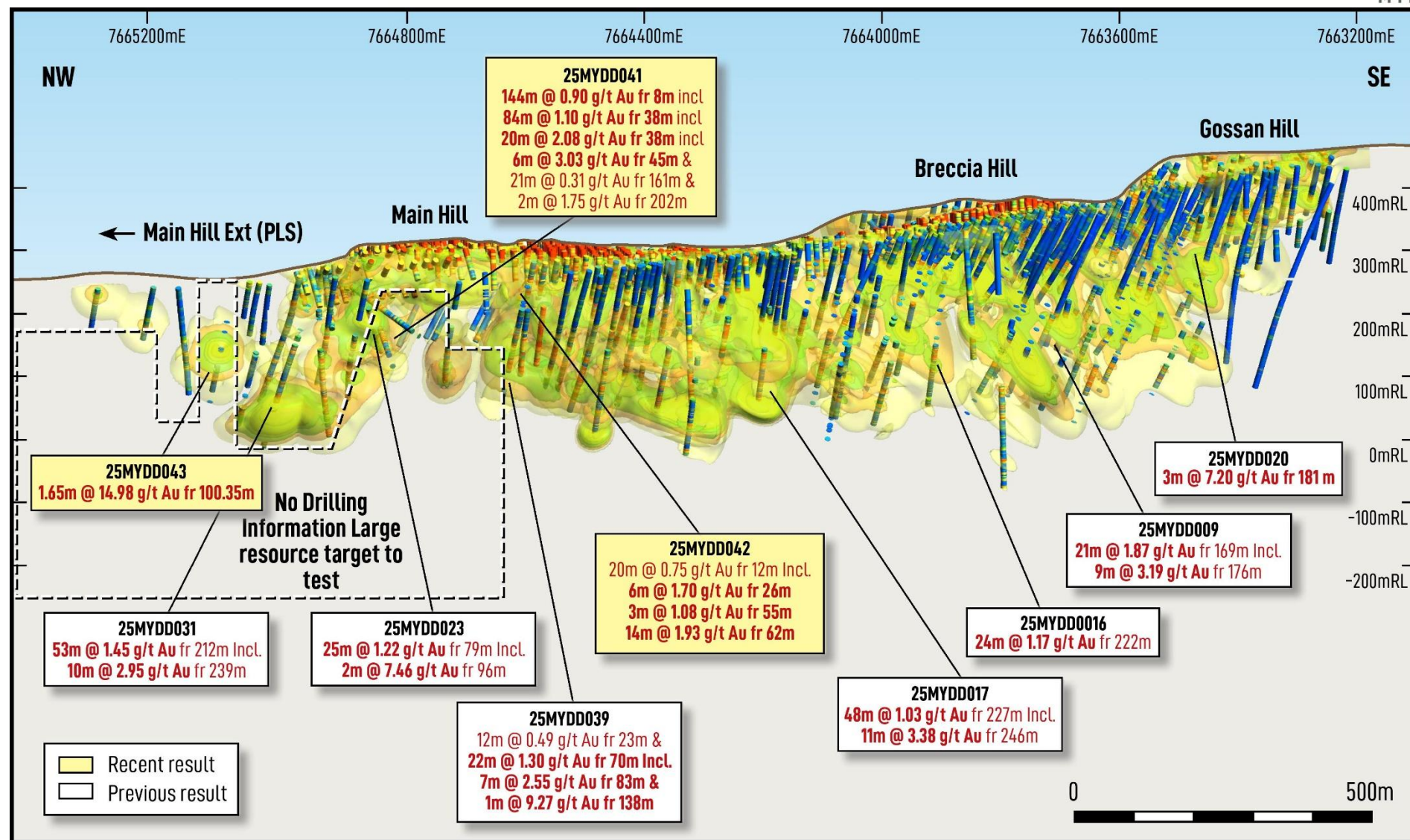
Figure 1. Leapfrog 'grade shell' model of the Main Trend showing significant current results (in yellow boxes) and historic holes (white boxes). Hole 25MYDD031 shows the position of the new 'Monster' Zone. The outer grade shell is >0.1 g/t Au. Looking northeast. Historic results are from drill results from ASX announcements dated 17 July & 6 August 2025.
