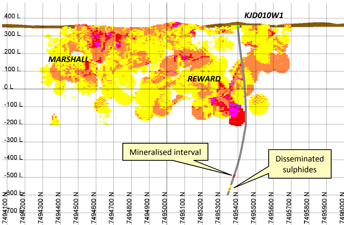
Figure 3 Marshall-Reward long section showing resource blocks and trace of KJD010W1 in grey. Yellow blocks 0.35-0.8% Cu, orange 0.8-2% Cu, red 2-3% Cu, magenta >3% Cu.
