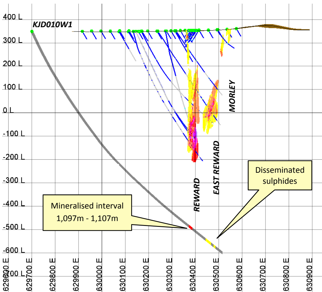
Figure 2 Reward Resource cross section showing location of mineralised intersections in KJD010W1.
