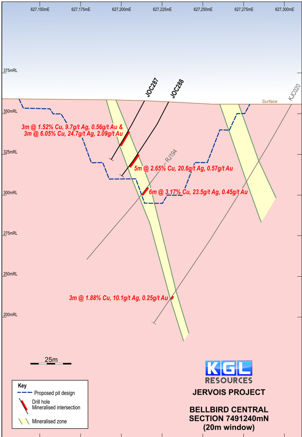
Figure 2 Bellbird Cross-Section
