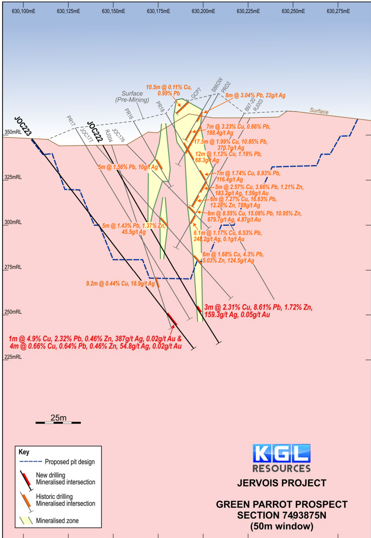
Figure 1 Green Parrot Cross-Section
