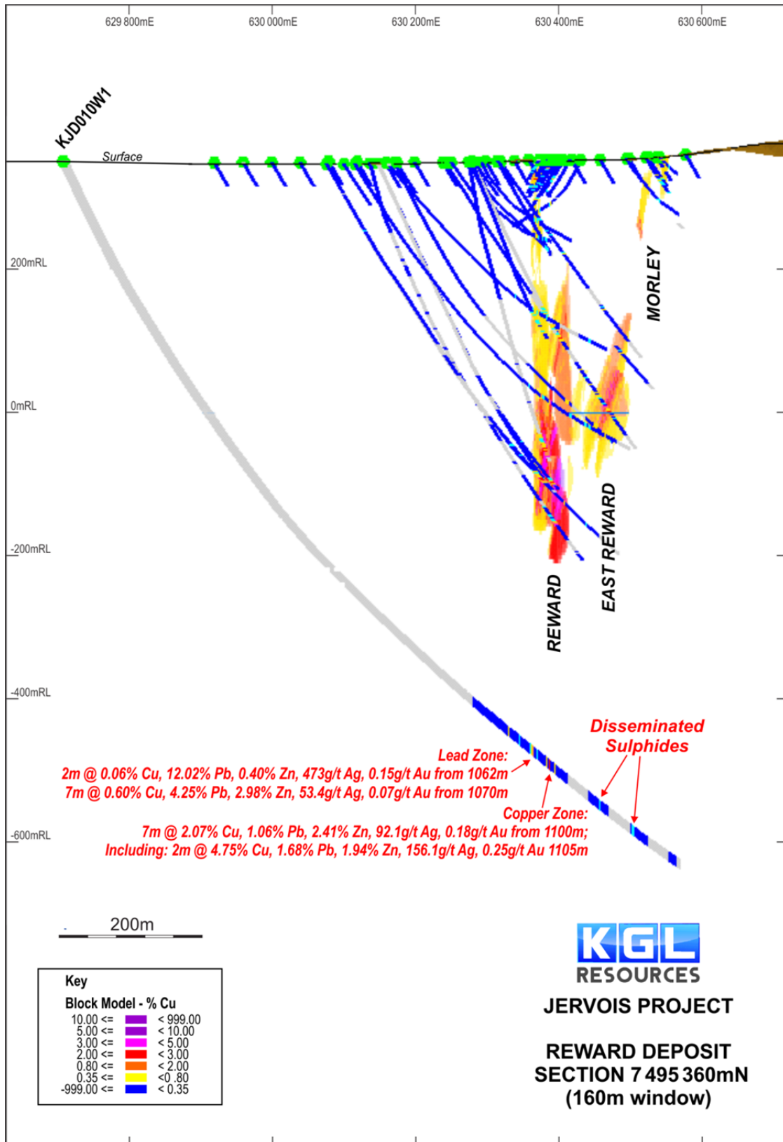
Figure 1 Reward Resource cross section showing location of mineralised intersections in KJD010W1. .
