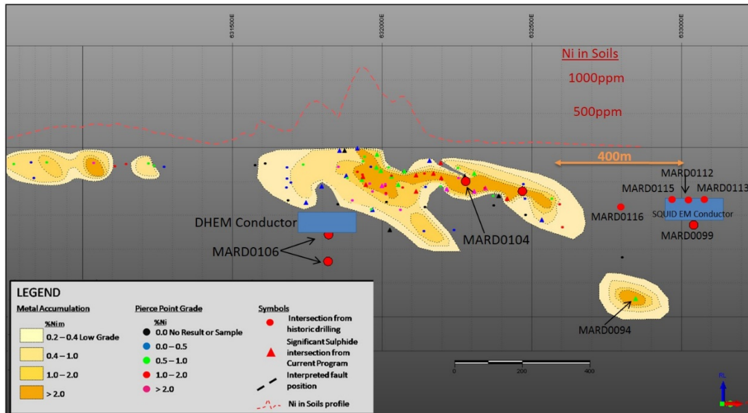
Figure 2: Long Section, looking to the Northwest showing the Ni accumulation (yellow shading), historic drill pierce points and the pierce points from the recently completed holes (Red spots). Blue rectangles indicate conductor plate models
