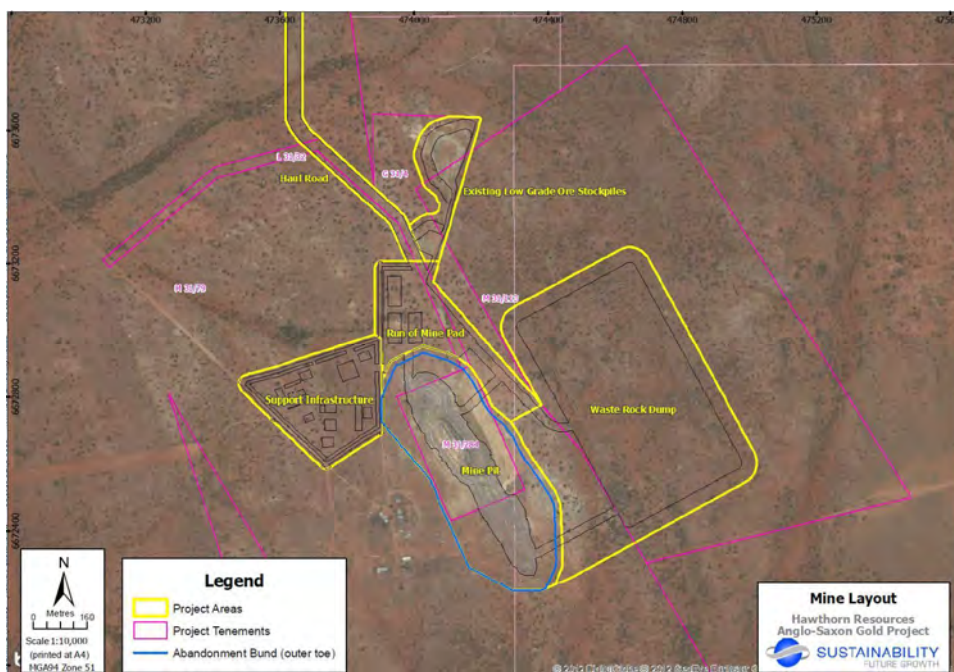
Figure 6. Anglo Saxon Deposit – Proposed Mine Layout
