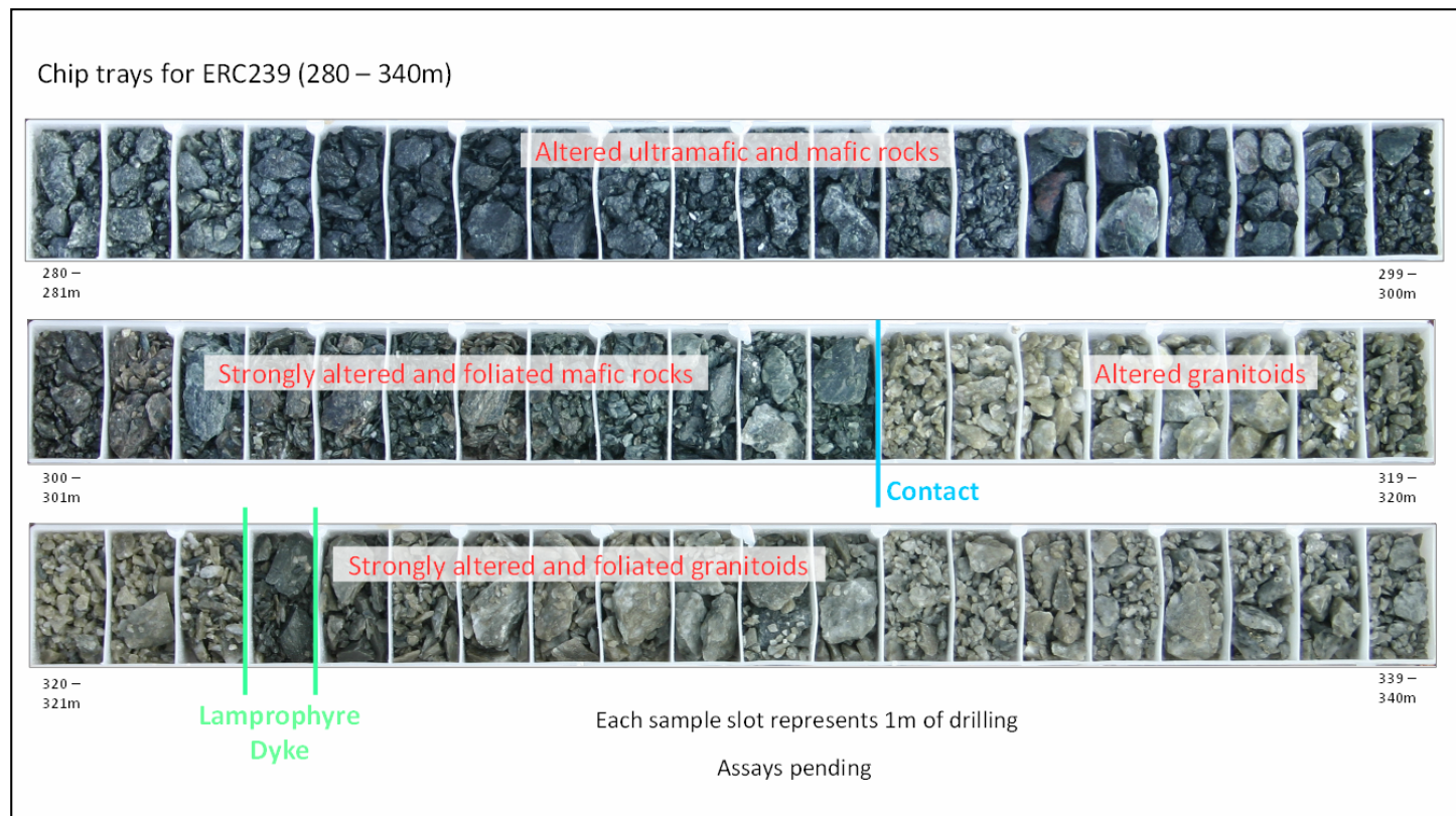
Fig. 7: Chip trays for step-out drill hole ERC239 (see Fig.6).
