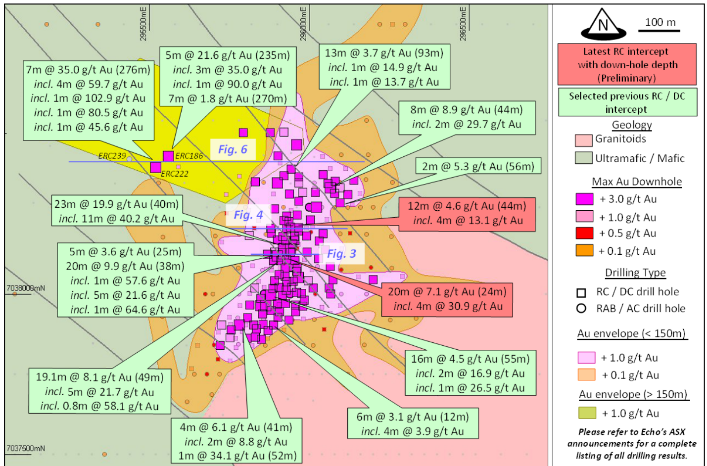
Fig. 2: Summary of drill intersections.
