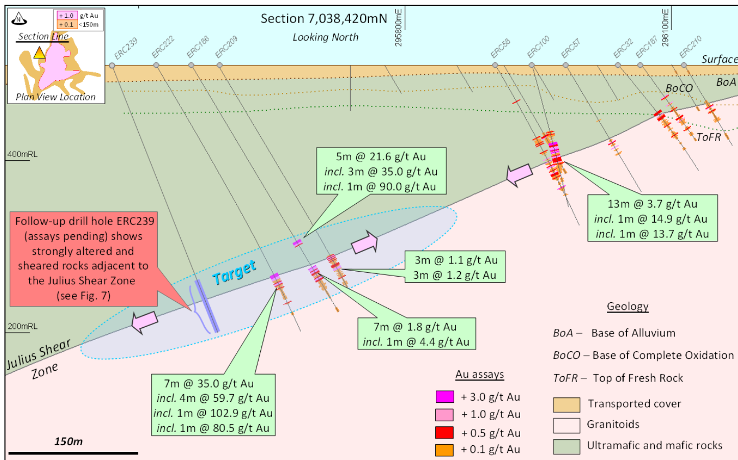
Fig. 6: Location of follow-up drill hole ERC239 (assays awaited) in relation to the high-grade gold intercepts in step-out drill holes ERC222 and ERC186.
