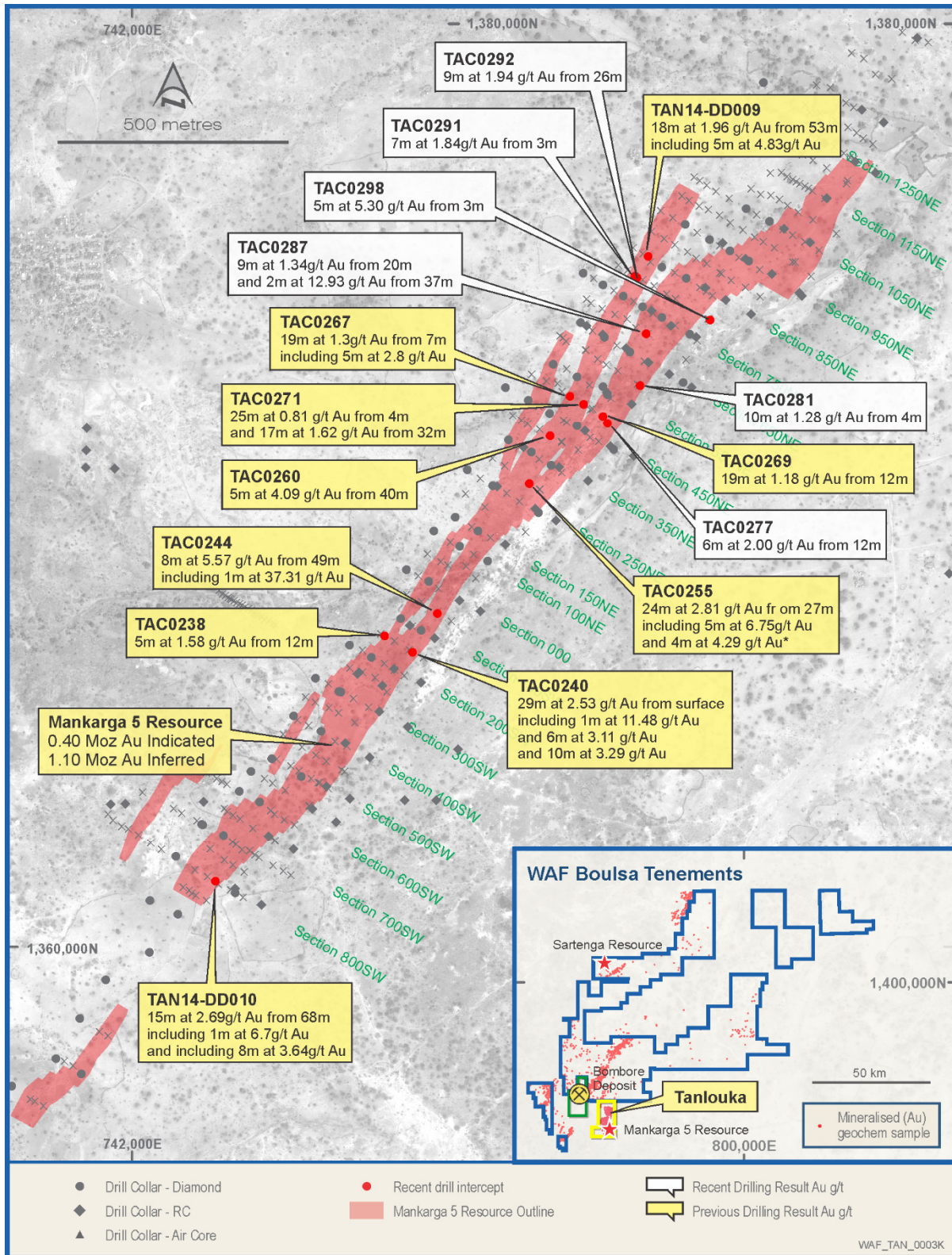
Figure 1: Mankarga Drilling Summary Plan
