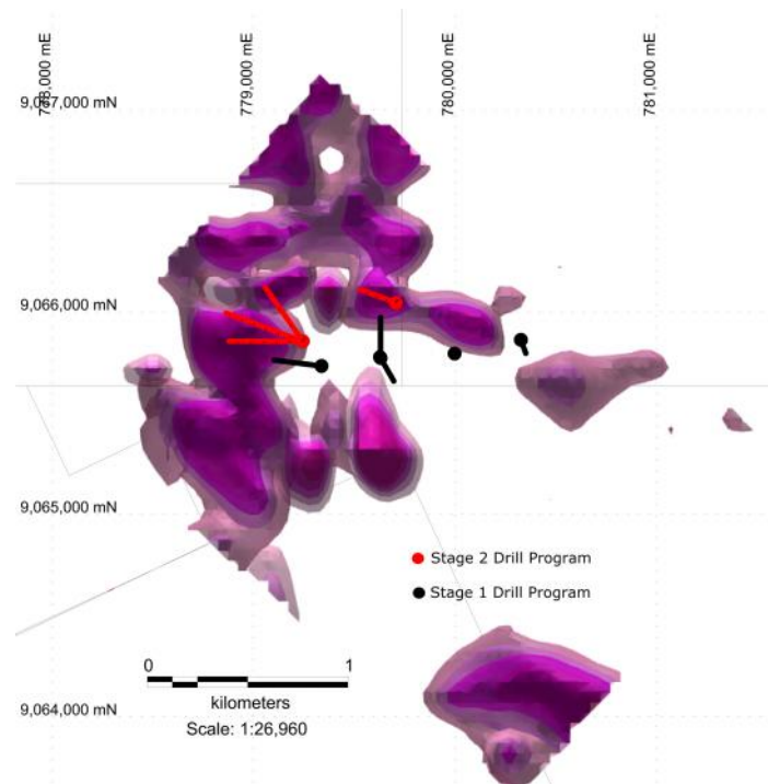
Figure 1 - Alumbre Project magnetic susceptibility 3D MVI model and the proposed Stage 2 drill program.”
