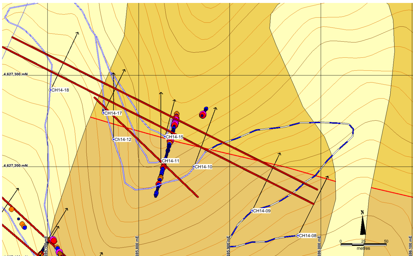
Figure 3 Copper Gold Zone (CGZ) map showing planned drill hole locations, roads in blue, planned roads dashed blue lines and mineralised zone in red
