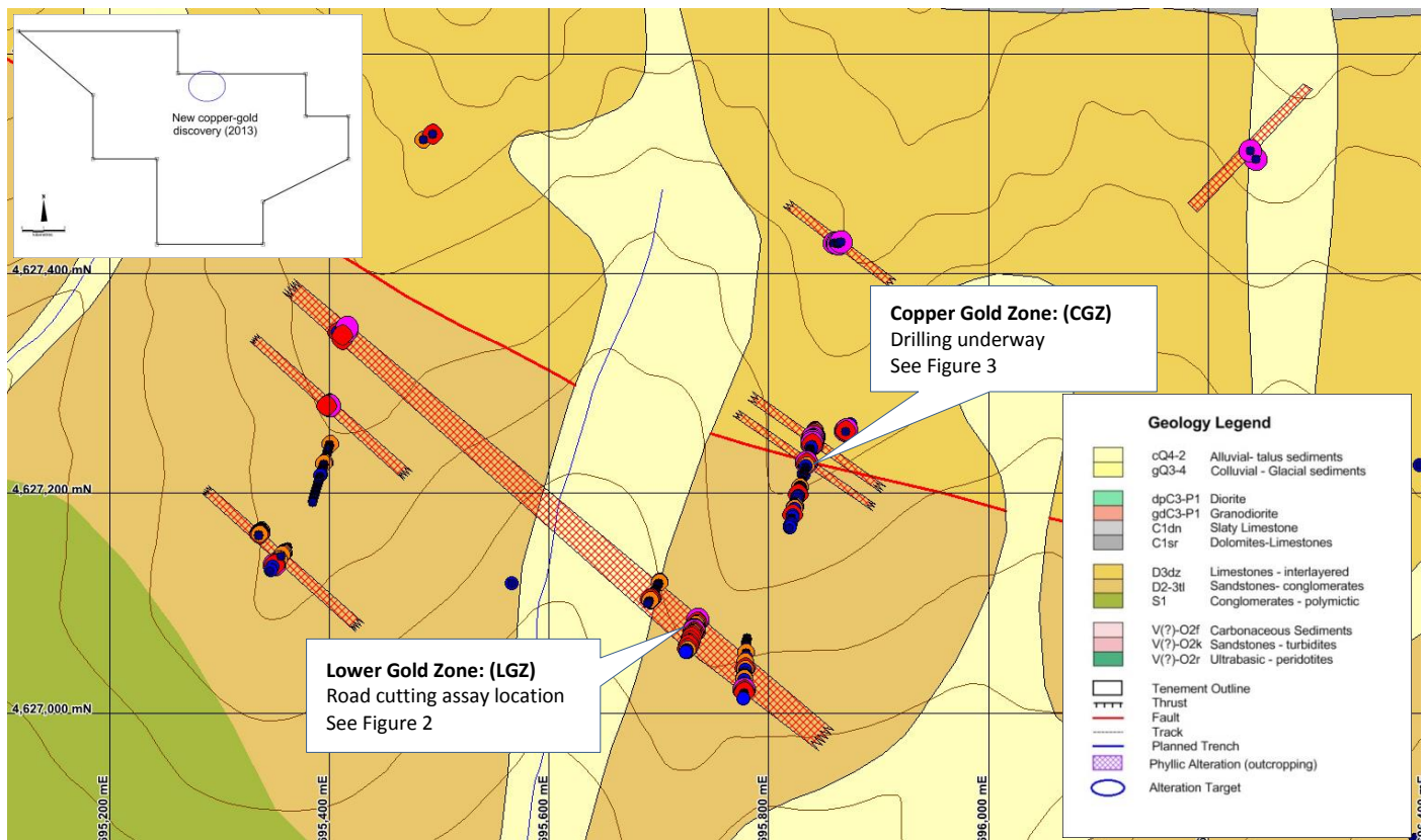
Figure 1 Interpreted mineralised zones (red hatched areas) with sampling and drilling locations.
