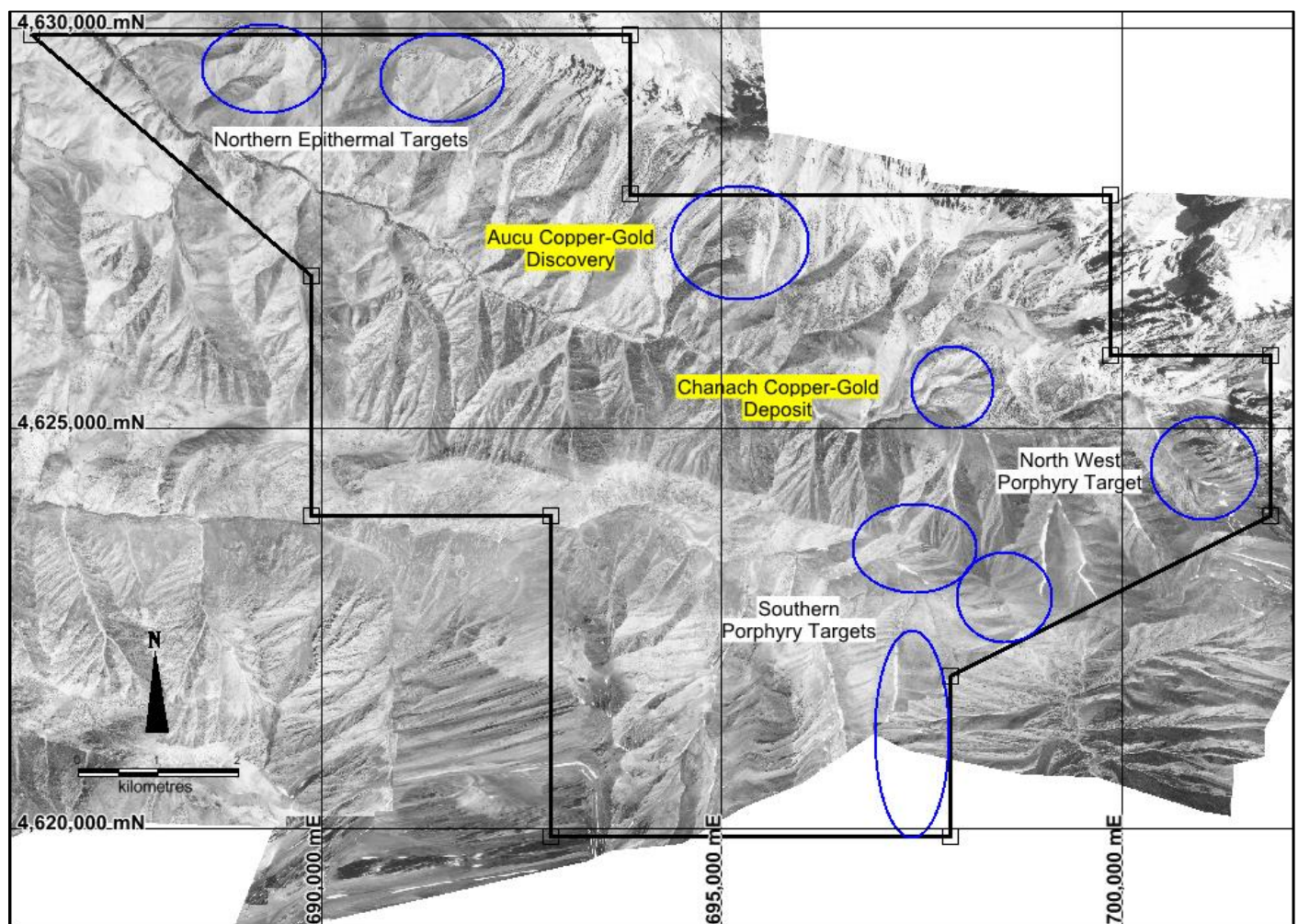
Figure 5 Map showing the location of the Aucu copper-gold discovery 2km to the NNW of the existing Chanach copper-gold deposit.
