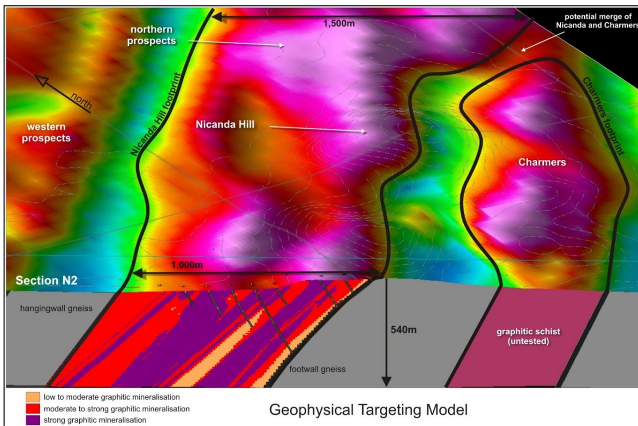
Figure 3. 3D cross section image of drill section N2 block model with VTEM draped on topography. This image is for illustrative purposes only and forms a part of a block model, which uses geostatistics to assess trends for better drill targeting.
