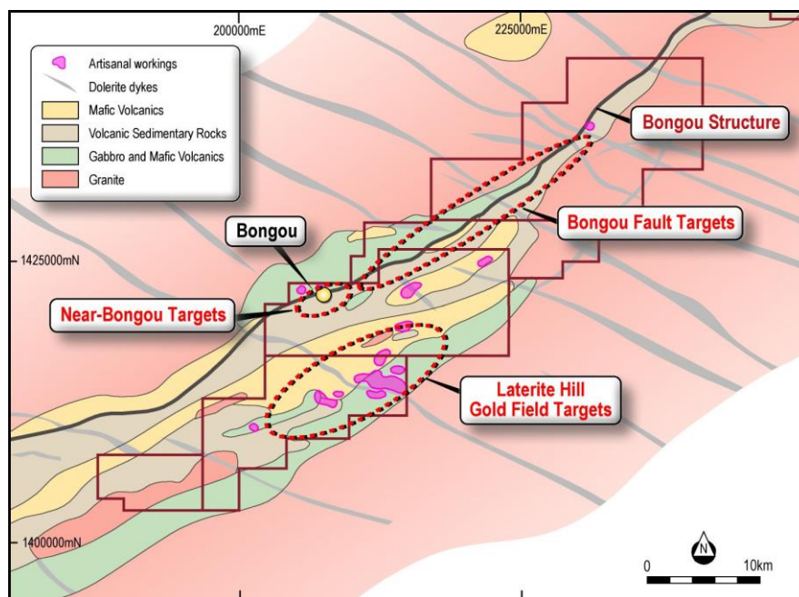
Figure 3: Geological map of SW Bonsiega permit group, including Bongou, showing PDI’s priority target areas for the discovery of additional high-grade gold resources.
