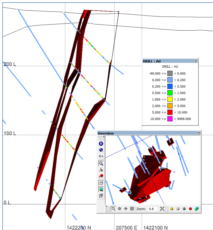
Figure 2: Cross-section of Bongou deposit showing mineralisation interpretation at 0.2 g/t Au
