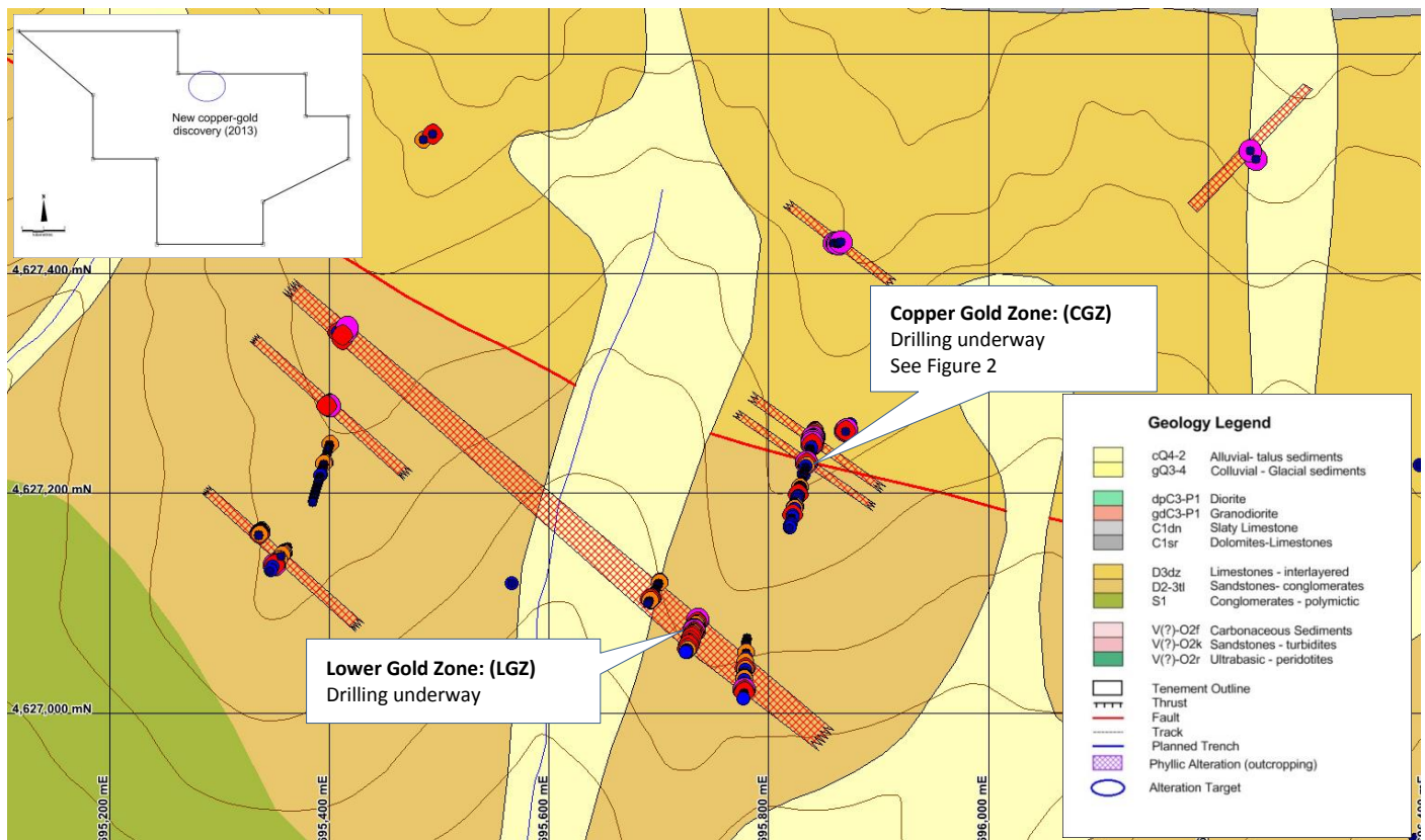
Figure 1 Interpreted mineralised zones (red hatched areas) with drilling locations.
