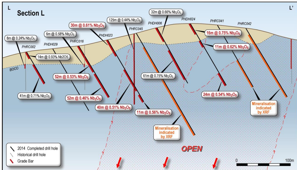
Figure 3: Section L with 2014 drillholes (thick black lines) showing previous results, significant new intercepts (red text), zones of mineralisation indicated by handheld XRF 3 with assays pending (orange bars) and historical drillholes and intercepts (grey lines and text).
