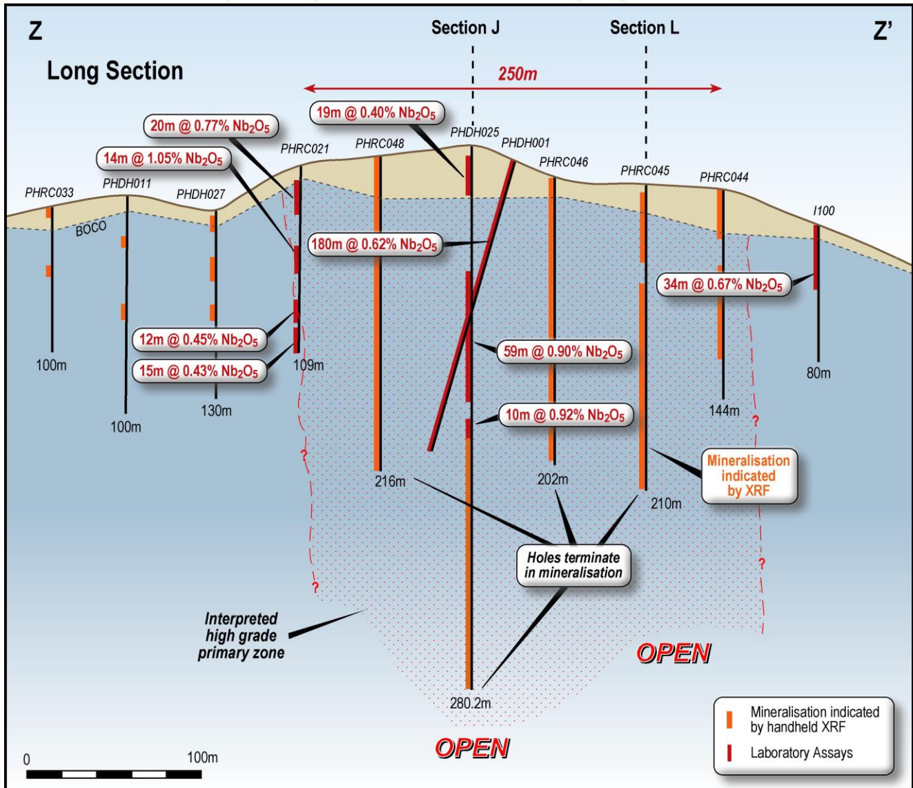
Figure 4: Long-Section showing projection of PHDH025 and the region of high-grade mineralisation indicated by recent RC drilling which has zones of high-grade mineralisation indicated by handheld XRF 3 with assays pending (orange bars).
