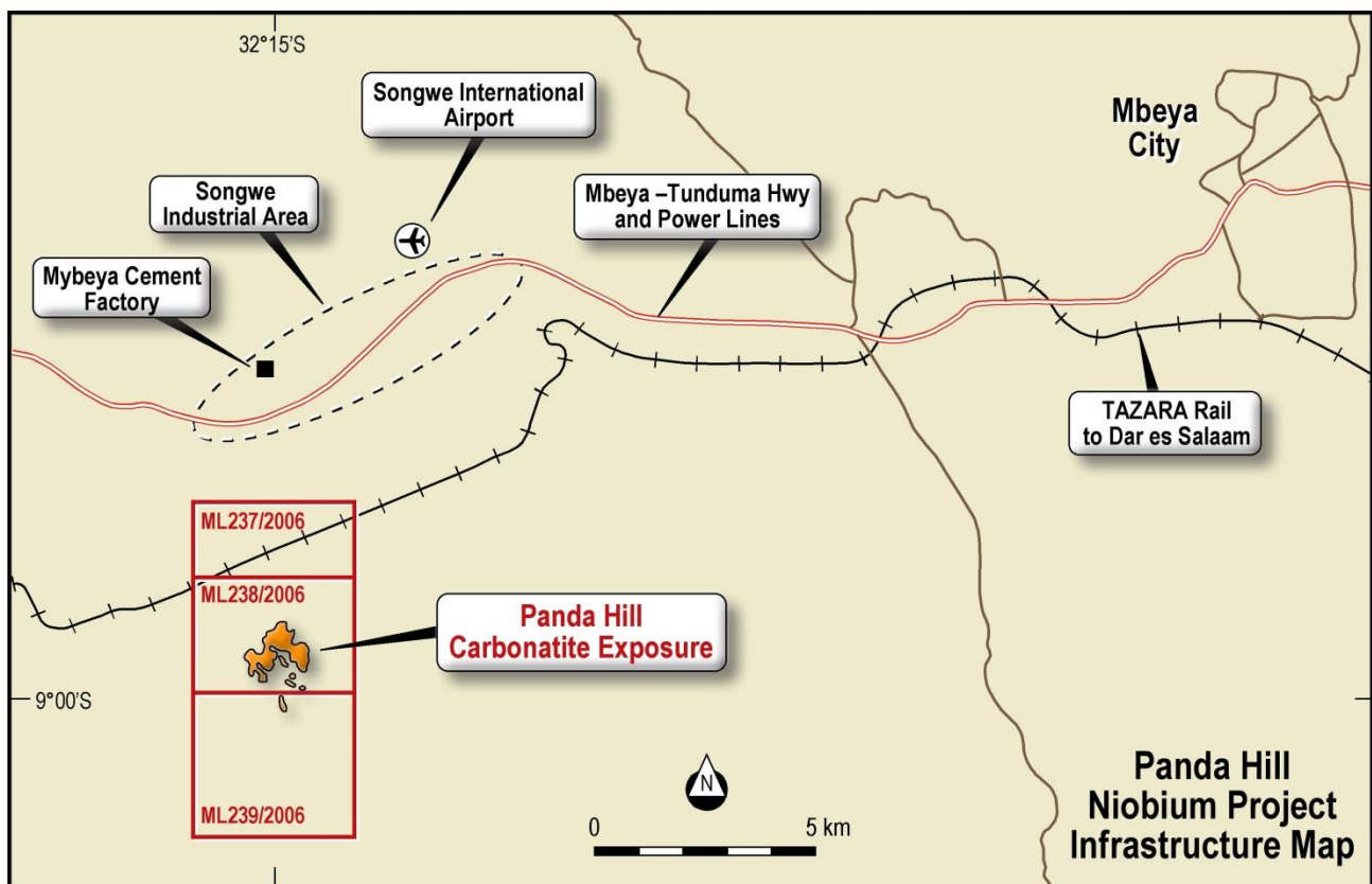
Figure 6: Location of the Project Tenure and Surrounding Infrastructure
