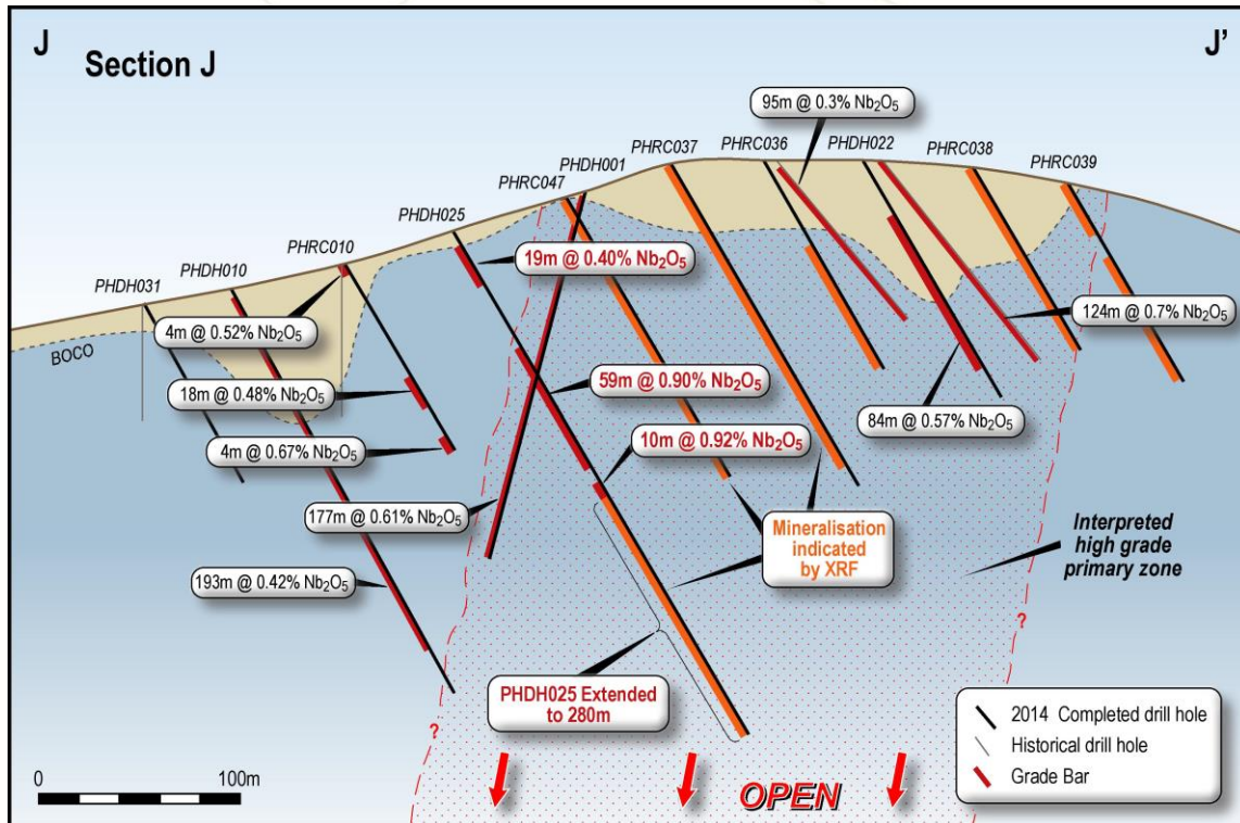
Figure 2: Section J with 2014 drillholes (thick black lines) showing previous results, significant new intercepts (red text), zones of mineralisation indicated by handheld XRF 3 with assays pending (orange bars) and historical drillholes and intercepts (grey lines and text).
