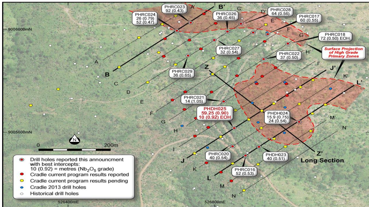
Figure 1: Panda Hill resource drilling grid showing the location of drill holes reported in this release, 2014 holes already reported (red) and holes with assays pending (yellow). Refer to section lines for subsequent figures. The approximate surface projection of emerging high-grade zones is shown in red shade. Other mineralised zones inside the resource area are omitted for clarity.
