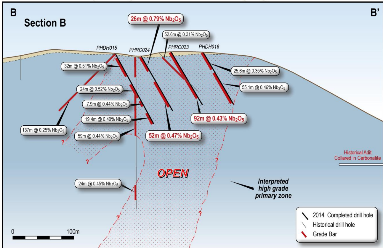
Figure 5: Section B in northern part of the drilling area showing 2014 drillholes (thick black lines) showing previous results, significant new intercepts (red text) and historical drillholes and intercepts (grey lines and text).
