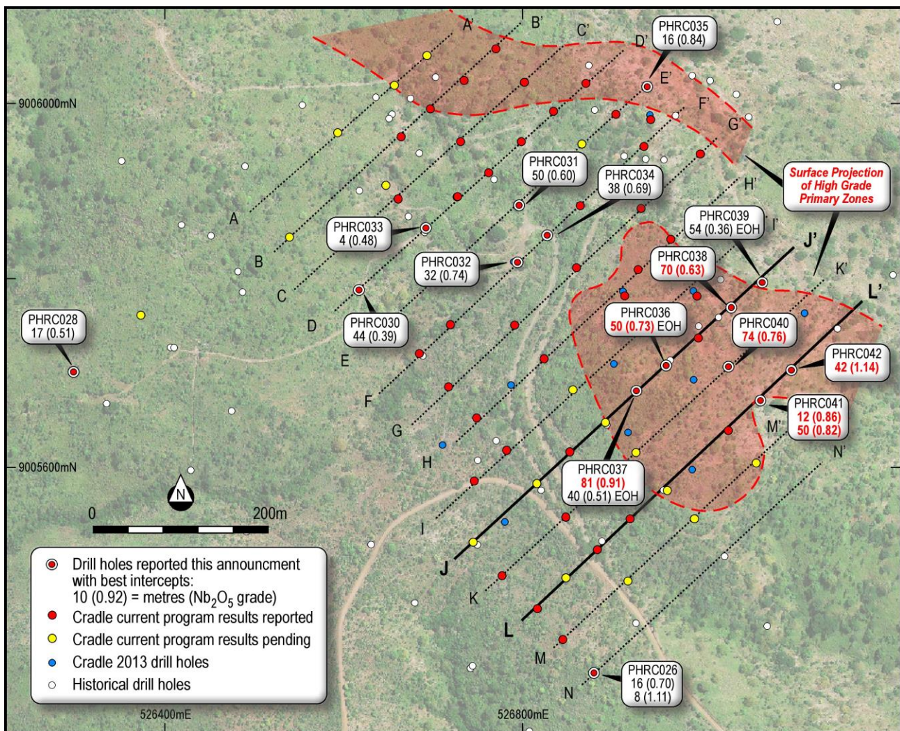
Figure 1: Panda Hill resource drilling grid showing the location of drill holes reported in this release, 2014 holes already reported (red) and holes with assays pending (yellow). Refer to section lines for subsequent figures. The approximate surface projection of the emerging high-grade zones is shown in red shade. Other mineralised zones inside the resource area are omitted for clarity.
