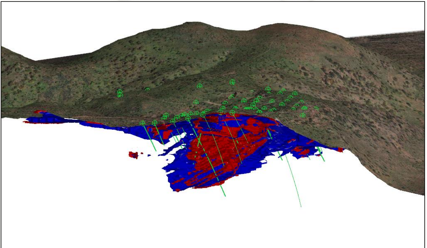
Figure 4: Preliminary mineralisation models showing the extent of the > 0.3% Nb 2 O 5 (blue) and >0.6% Nb 2 O 5 (red) regions.
