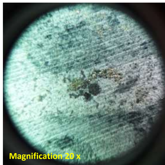
Figure 2 – (Drill Depth 49.85m) veinlet of quartz-pyrite molybdenite with trace chalcopyrite.
