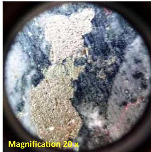
Figure 3 - veinlet of pyrite-chalcopyrite with biotite halo (2mm).
