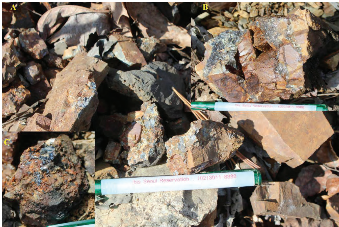
Figure 9: Composite photo showing sulphide mineralisation on hydraulic fractures within the conglomerate (A), chalcopyrite and pyrrhotite mineralisation (B) and galena (C).
