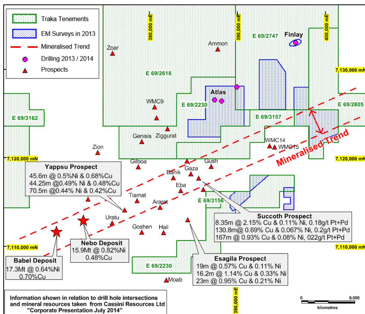
Figure 3: Tenement location plan in the Jameson area showing prospect locations and a selective number of drillhole intersections
