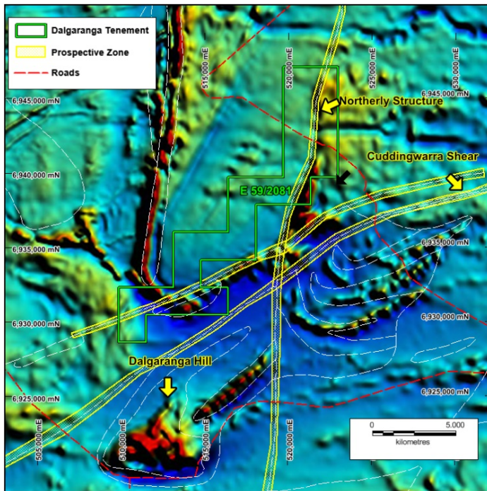
Figure 6: Aeromagnetic image of Dalgaranga area showing tenement location
