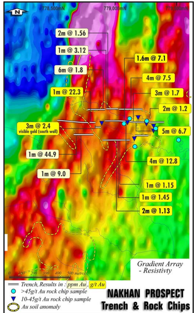
Figure 4. Summary Map for Nakhan Prospect within Sayabouly Concession Area with rock chip and trench results
