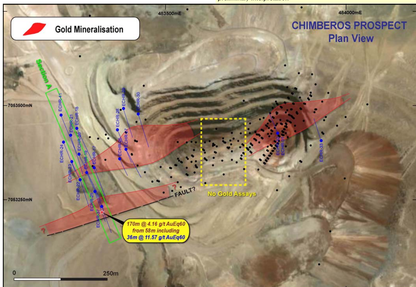
Figure 3. Plan of Chimberos recent drilling intersections and preliminary interpretation
