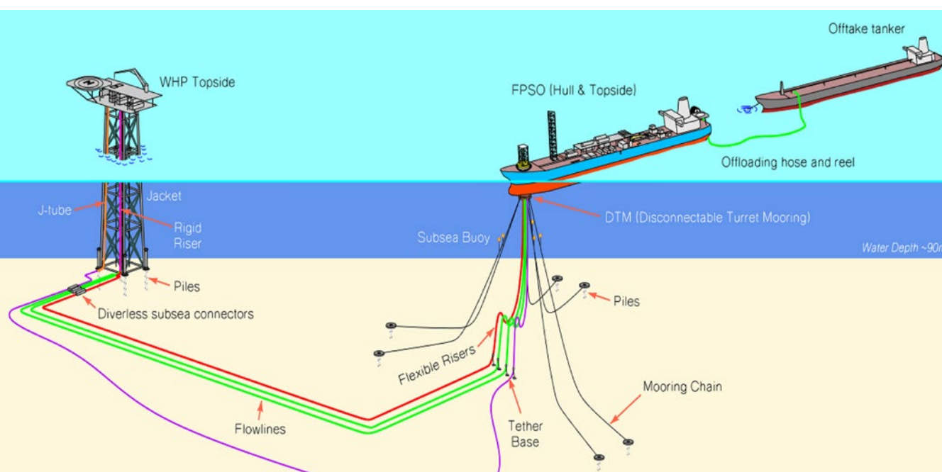
Figure 2. Proposed Dorado Field Development Layout.
