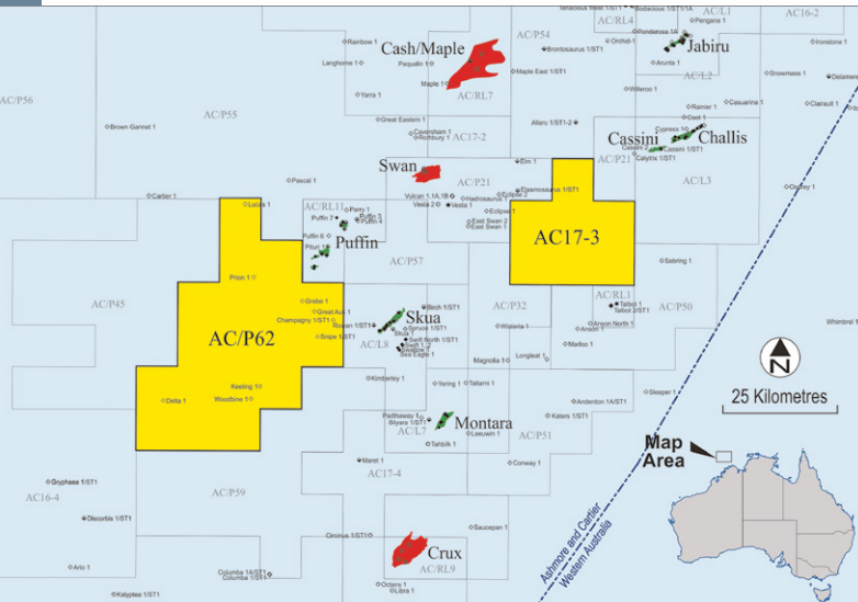
Figure 7. Outline of the AC/P62 and AC/P63 permits in relation to existing fields.
