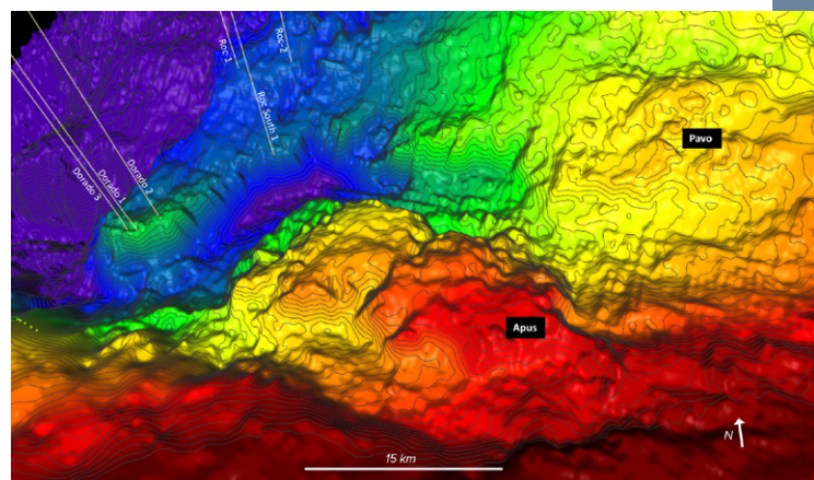
Figure 3. Map of top Caley/TR15 with well locations and significant prospects in the Bedout Sub-basin.
