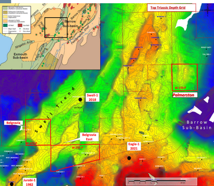
Figure 5. Top Triassic map of Belgravia and Palmerston prospects within WA-155-P.
