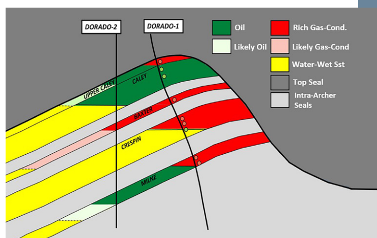
Figure 1. Schematic image of the Dorado field and Dorado-1 and Dorado-2 well locations.
