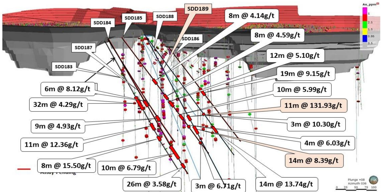
Figure 1 – Long-section of Smarts Underground looking north-east illustrating key recent intersections. SDD189 intersections are highlighted.
