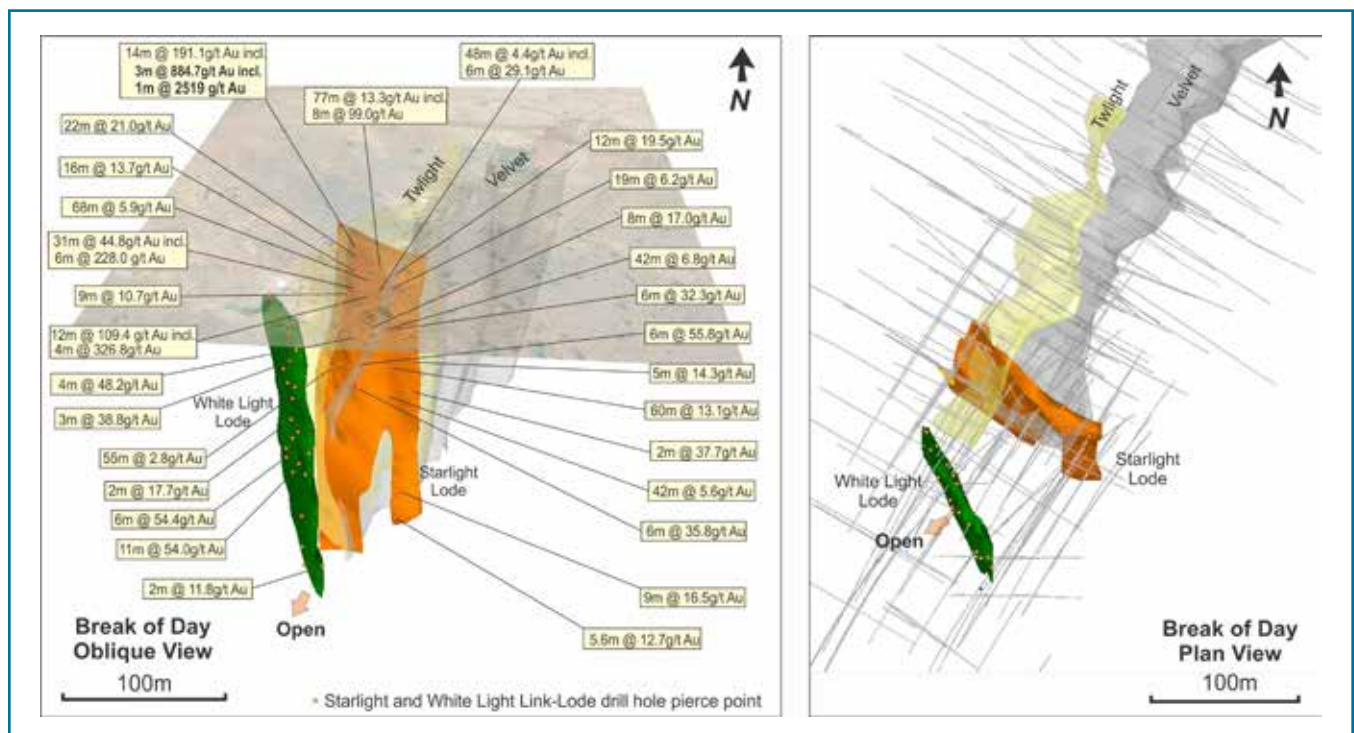
Figure 2: Schematic 3D model showing Starlight and White Light lodes at Break of Day, Cue Project
