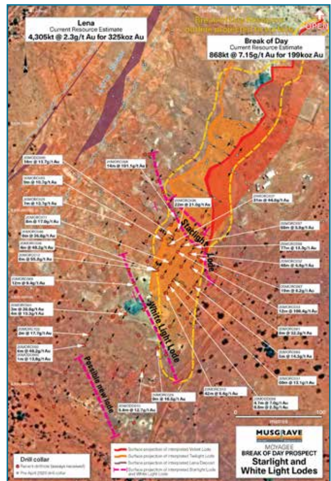
Figure 3: Plan showing Starlight and White Light lodes and recent drill collars at Break of Day, Cue Project
