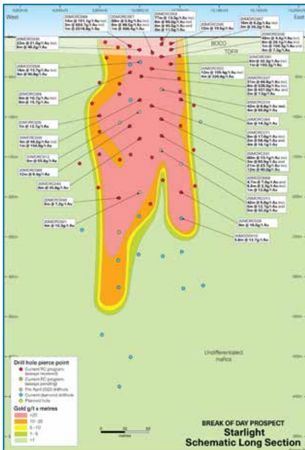
Figure 5: Long section of the Starlight lode, Break of Day, Cue Project showing select drill hole assays
