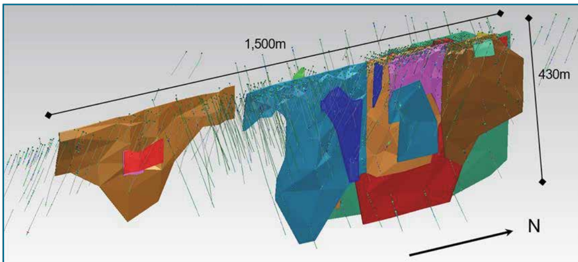
Figure 7: Lena Long section schematic showing current resource boundary of the 16 gold lodes and the opportunity at depth to extend the resource.
