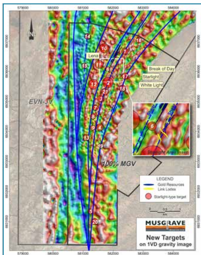
Figure 10: Regional gravity image showing new Starlight 'like' analogue targets, Cue Project
