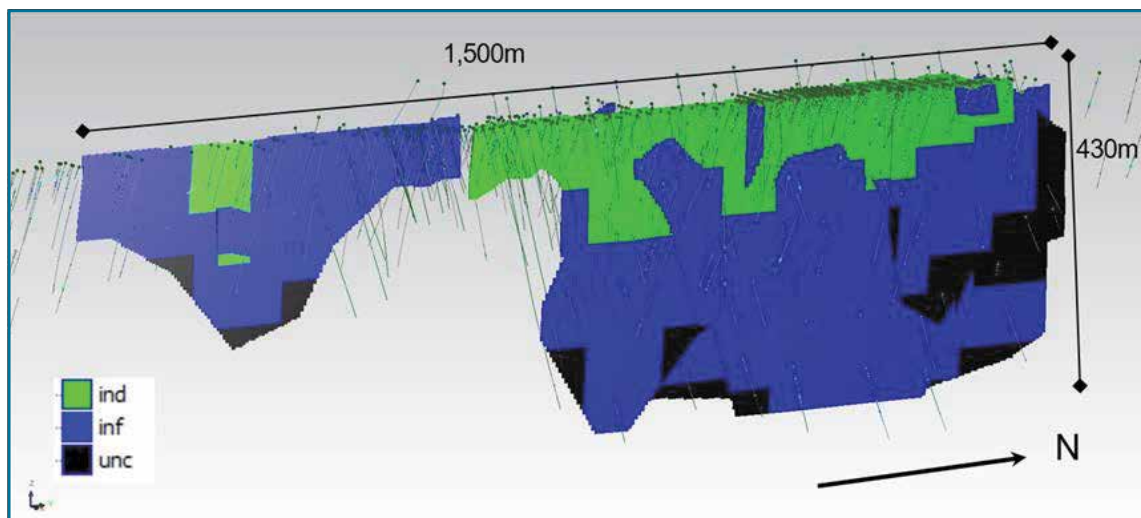
Figure 8: Lena long section block model showing resource classifications (Indicated Resources in green and Inferred Resources in blue. The black zones are unclassified).
