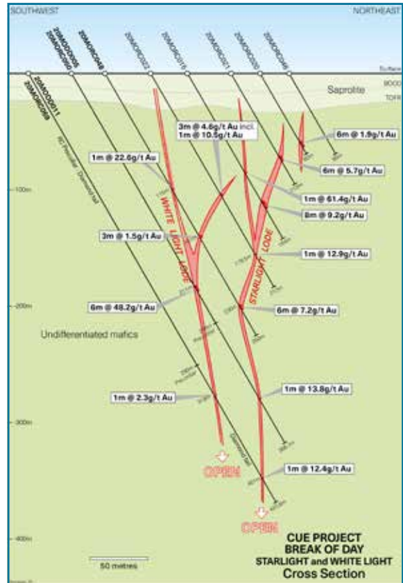
Figure 4: Cross sections showing Starlight and White Light lodes at Break of Day, Cue Project
