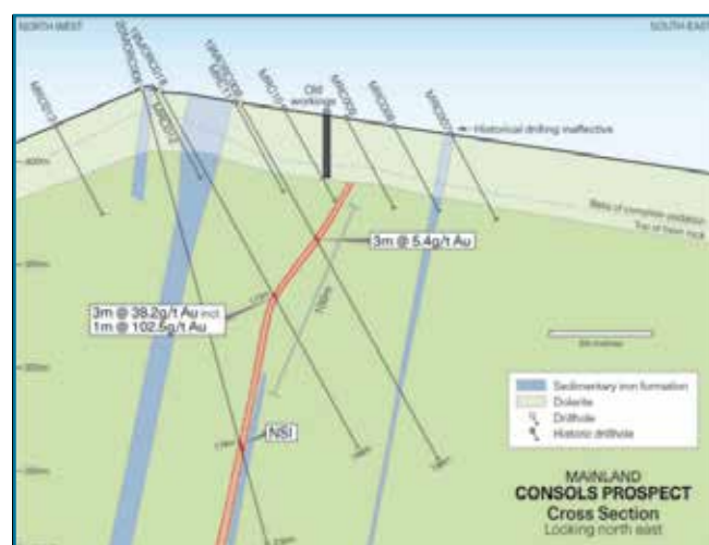
Figure 9: Geological cross section from the Consols Prospect, Mainland
