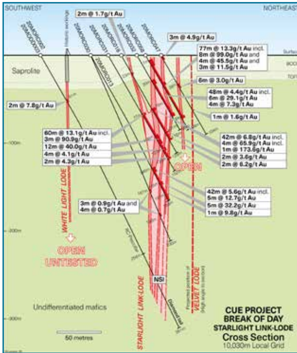
Figure 4: Cross sections showing Starlight and White Light lodes at Break of Day, Cue Project
