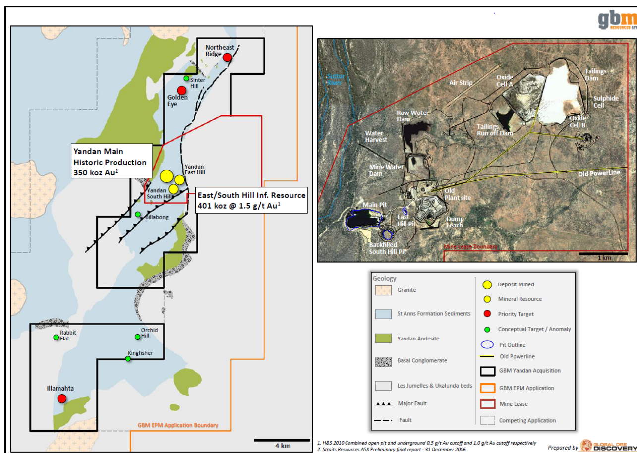
Figure 2: Yandan Gold Project and Mine Infrastructure
