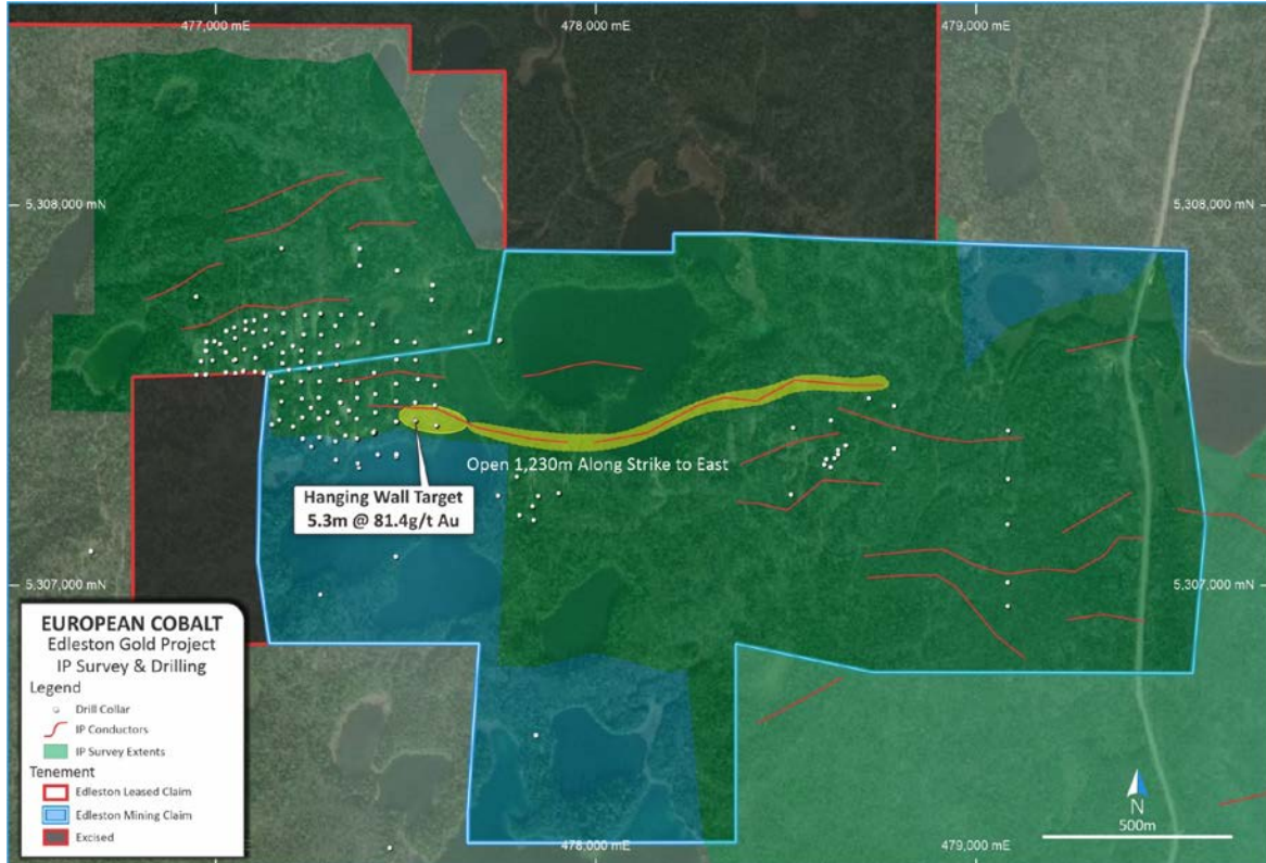
Figure 4: Edleston Hangingwall Target, IP Conductors & Drilling
