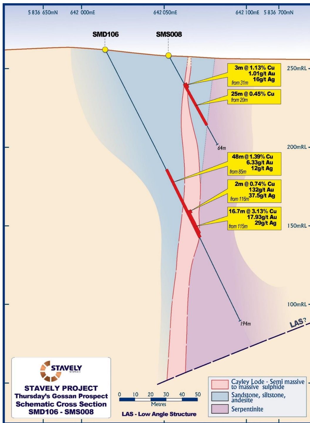
Figure 4. Drill hole SMD106 cross-section.
