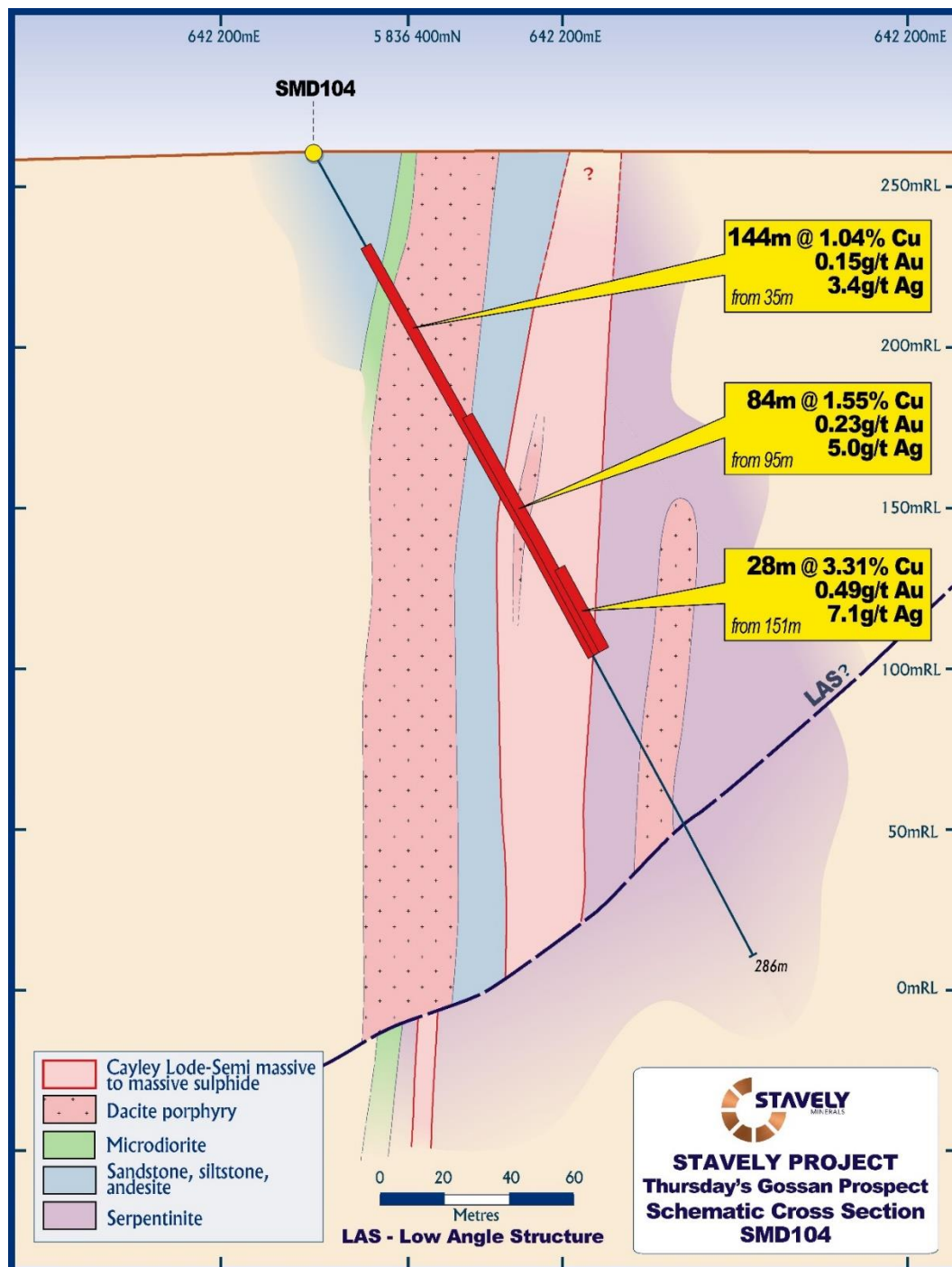
Figure 5. Drill hole SMD104 cross-section.
