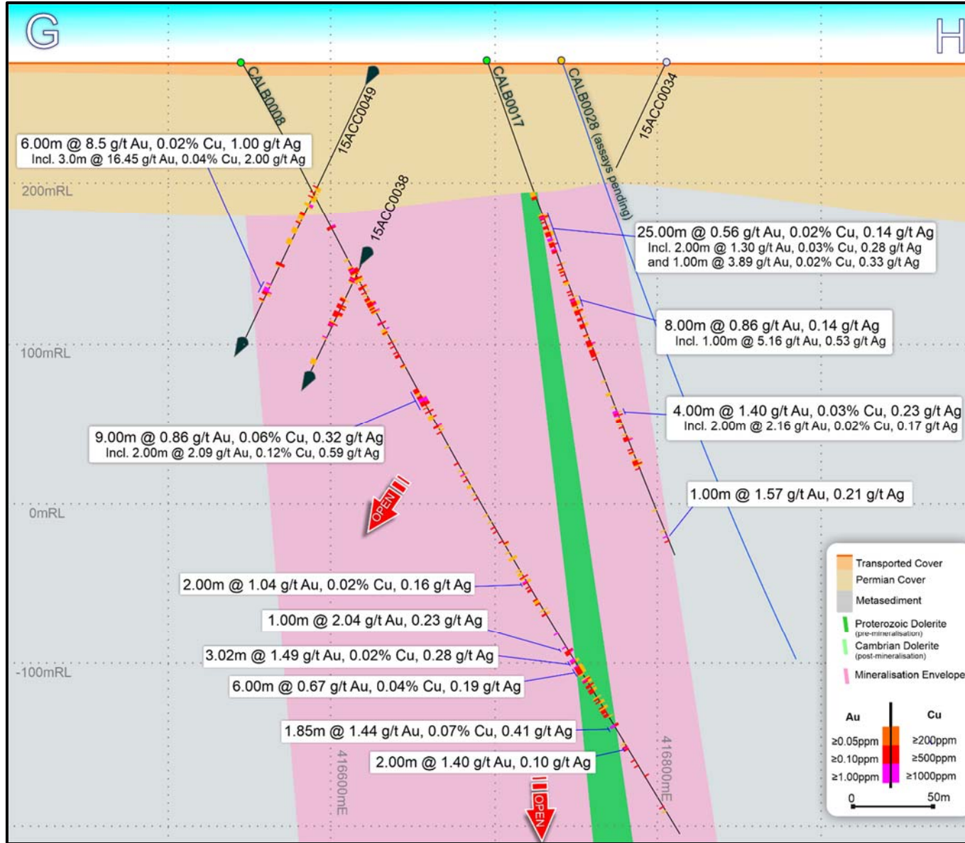
Figure 6: Calibre Deposit interpreted cross-section showing drill hole Au-Cu-Ag intersections including CALB0017. NB: 200m horizontal x 100m vertical grid – Approx. north looking.
