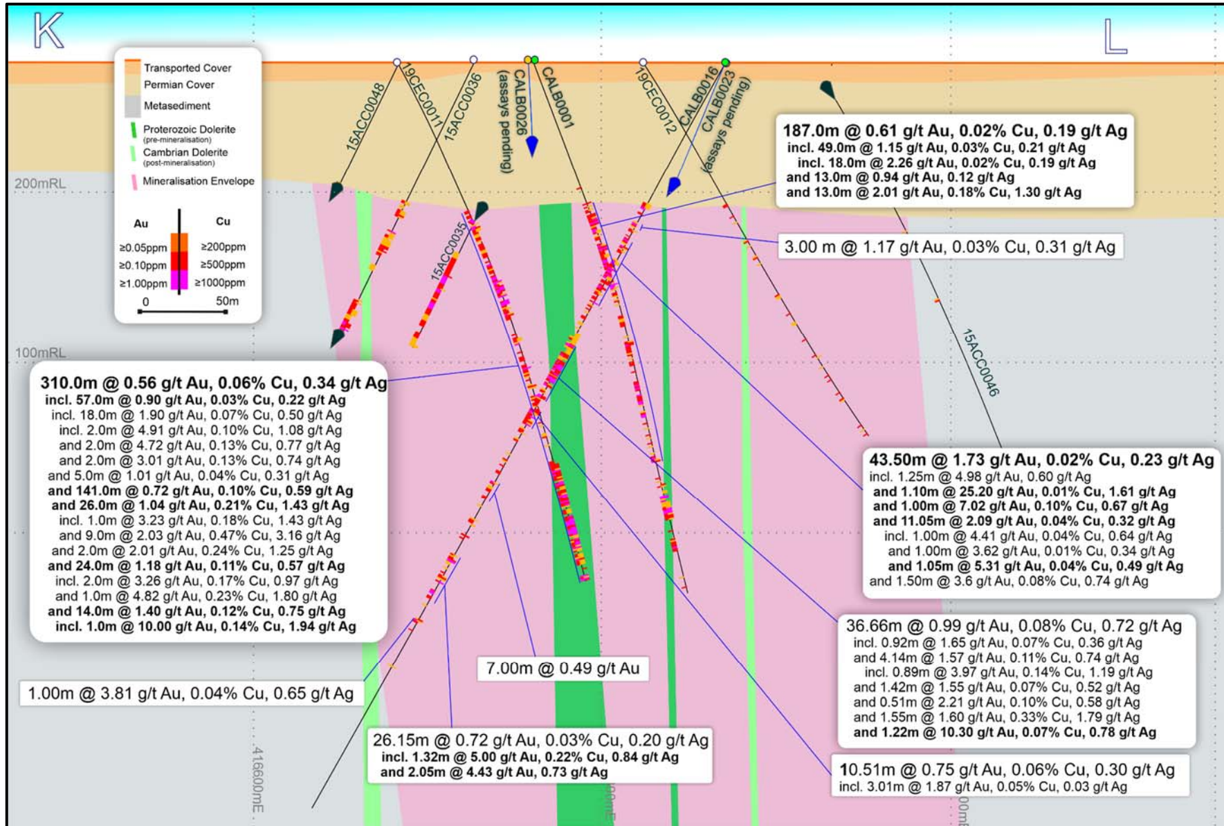
Figure 5: Calibre Deposit interpreted cross-section showing drill hole Au-Cu-Ag intersections including CALB0016. NB: 200m horizontal x 100m vertical grid – Approx. north looking.
