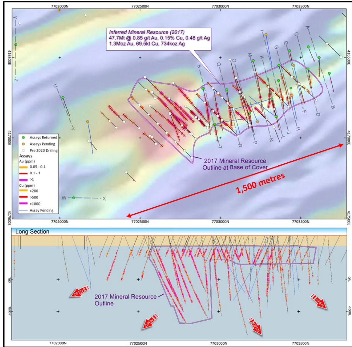
Figure 2: Calibre Deposit Plan over aeromagnetic image and west looking Vertical Projection showing all Calibre drill (including 2020) holes and depicting gold and copper grade distribution. NB: 500m horizontal x 200m vertical grid MGA Zone 51 / GDA 2020 grid.
