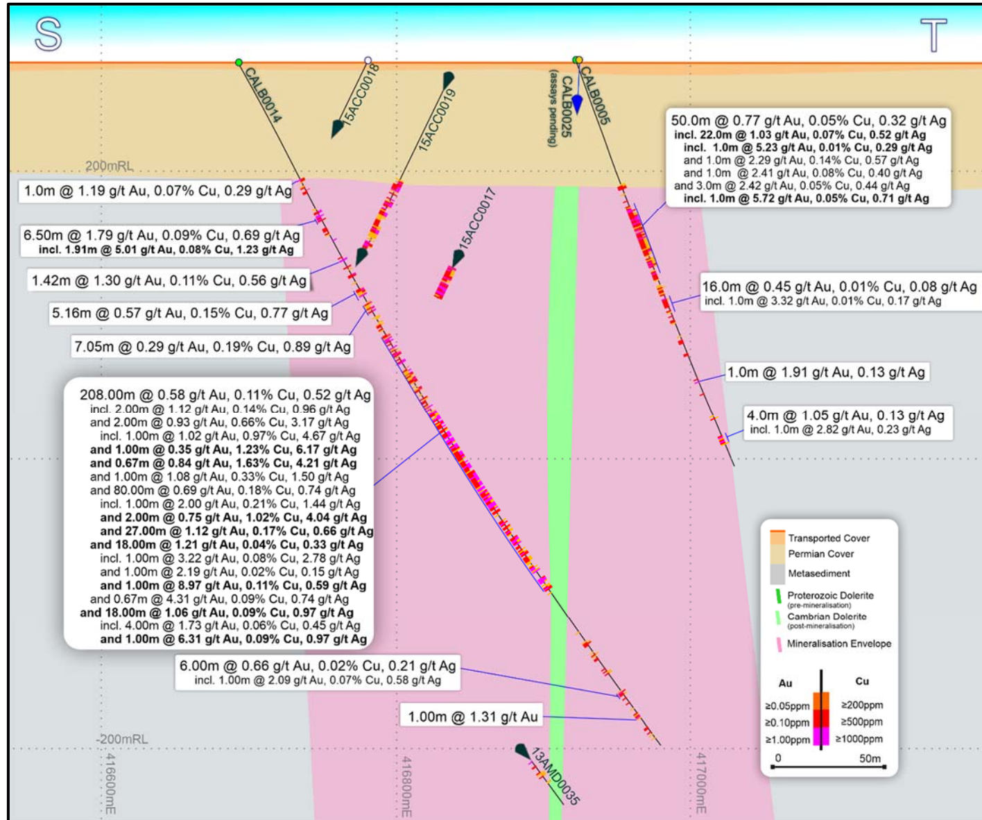
Figure 3: Calibre Deposit interpreted cross-section showing drill hole Au-Cu-Ag intersections including CALB0005 and CALB0014. NB: 200m horizontal x 100m vertical grid – Approx. north looking.
