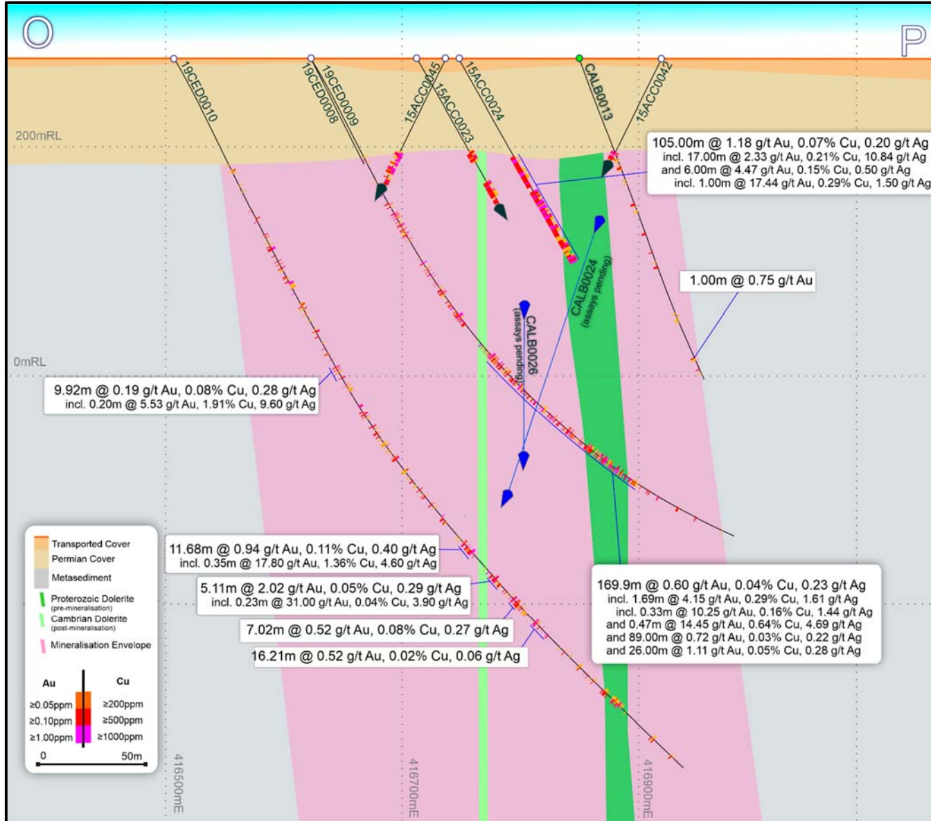
Figure 4: Calibre Deposit interpreted cross-section showing drill hole Au-Cu-Ag intersections including CALB0013. NB: 200m horizontal x 100m vertical grid – Approx. north looking.
